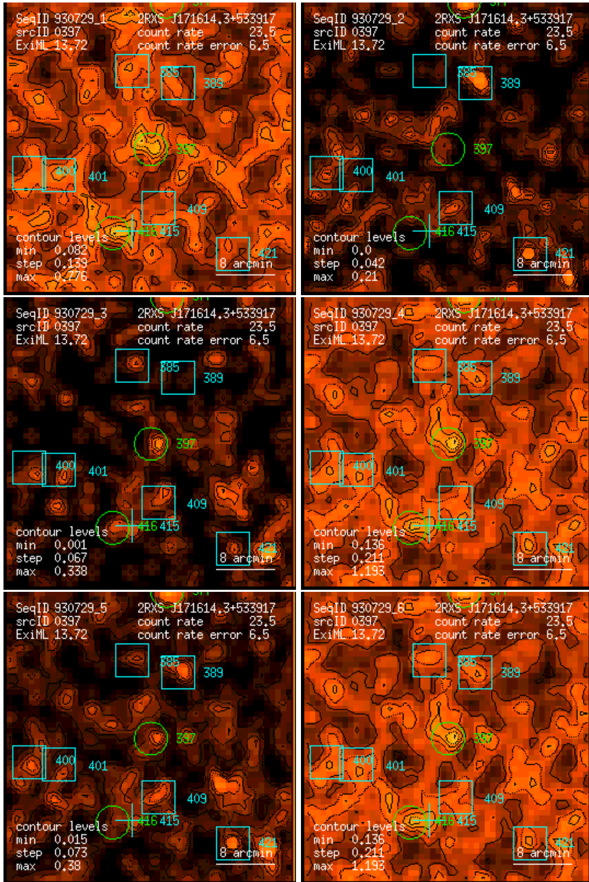
Figure 397: RASS 930729: detection 0397: band rate images, Gaussian filter: (1) PSPC channels 11 – 41, (2) 52 – 90, (3) 91 – 201, (4) 11 – 235, (5) 52 – 201, (6) 11 – 201. Broad band rates in counts/ks. Band rate contour levels in counts/ks/arcmin 2 .
