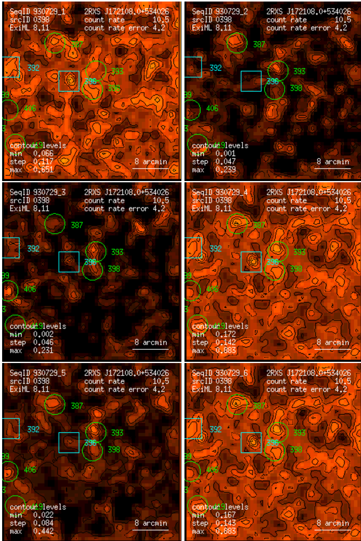
Figure 398: RASS 930729: detection 0398: band rate images, Gaussian filter: (1) PSPC channels 11 – 41, (2) 52 – 90, (3) 91 – 201, (4) 11 – 235, (5) 52 – 201, (6) 11 – 201. Broad band rates in counts/ks. Band rate contour levels in counts/ks/arcmin 2 .
