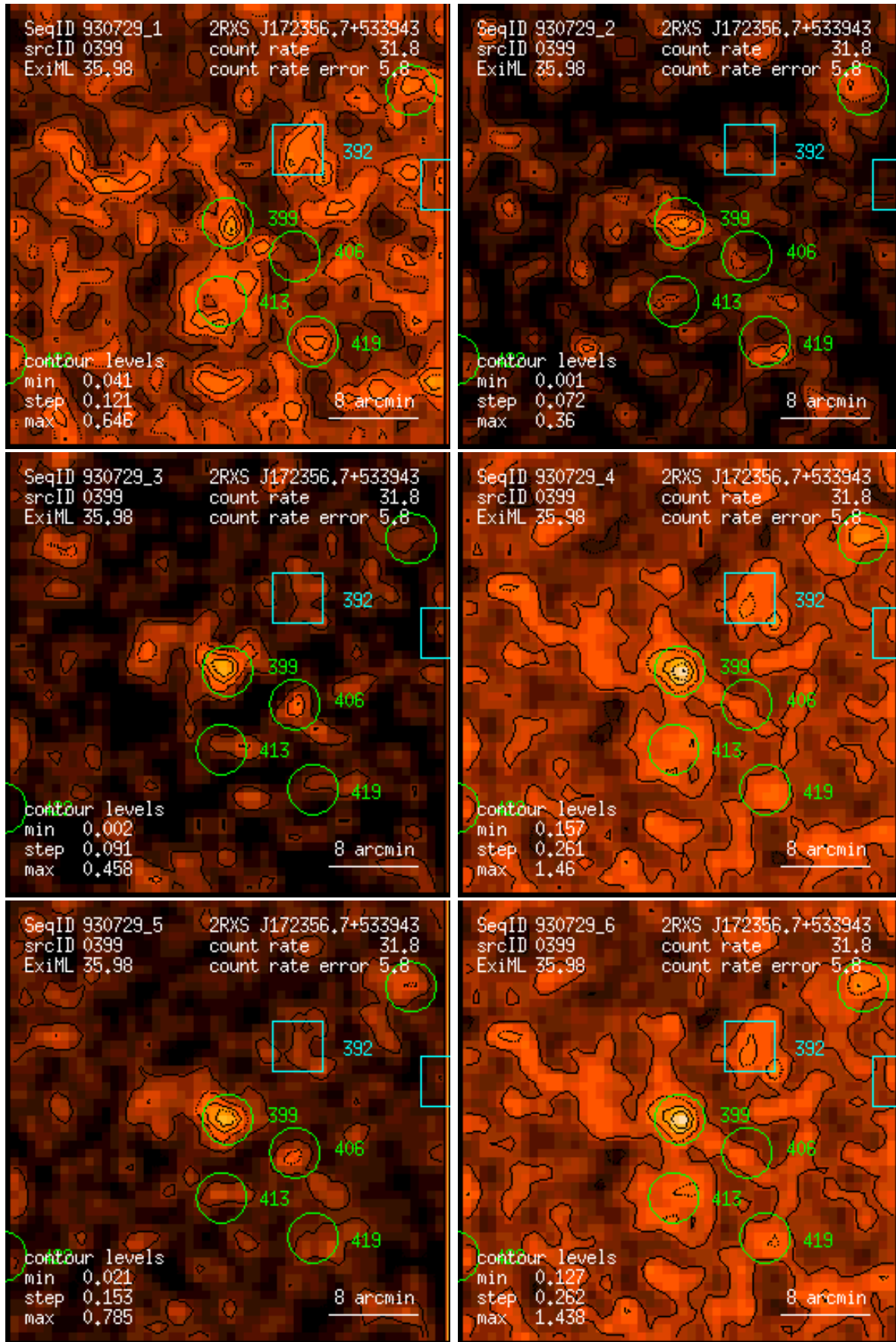
Figure 399: RASS 930729: detection 0399: band rate images, Gaussian filter: (1) PSPC channels 11 – 41, (2) 52 – 90, (3) 91 – 201, (4) 11 – 235, (5) 52 – 201, (6) 11 – 201. Broad band rates in counts/ks. Band rate contour levels in counts/ks/arcmin 2 .
