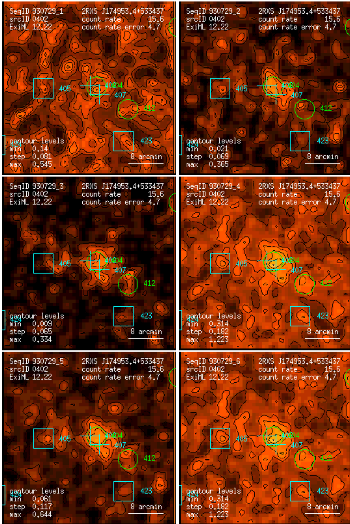
Figure 402: RASS 930729: detection 0402: band rate images, Gaussian filter: (1) PSPC channels 11 – 41, (2) 52 – 90, (3) 91 – 201, (4) 11 – 235, (5) 52 – 201, (6) 11 – 201. Broad band rates in counts/ks. Band rate contour levels in counts/ks/arcmin 2 .
