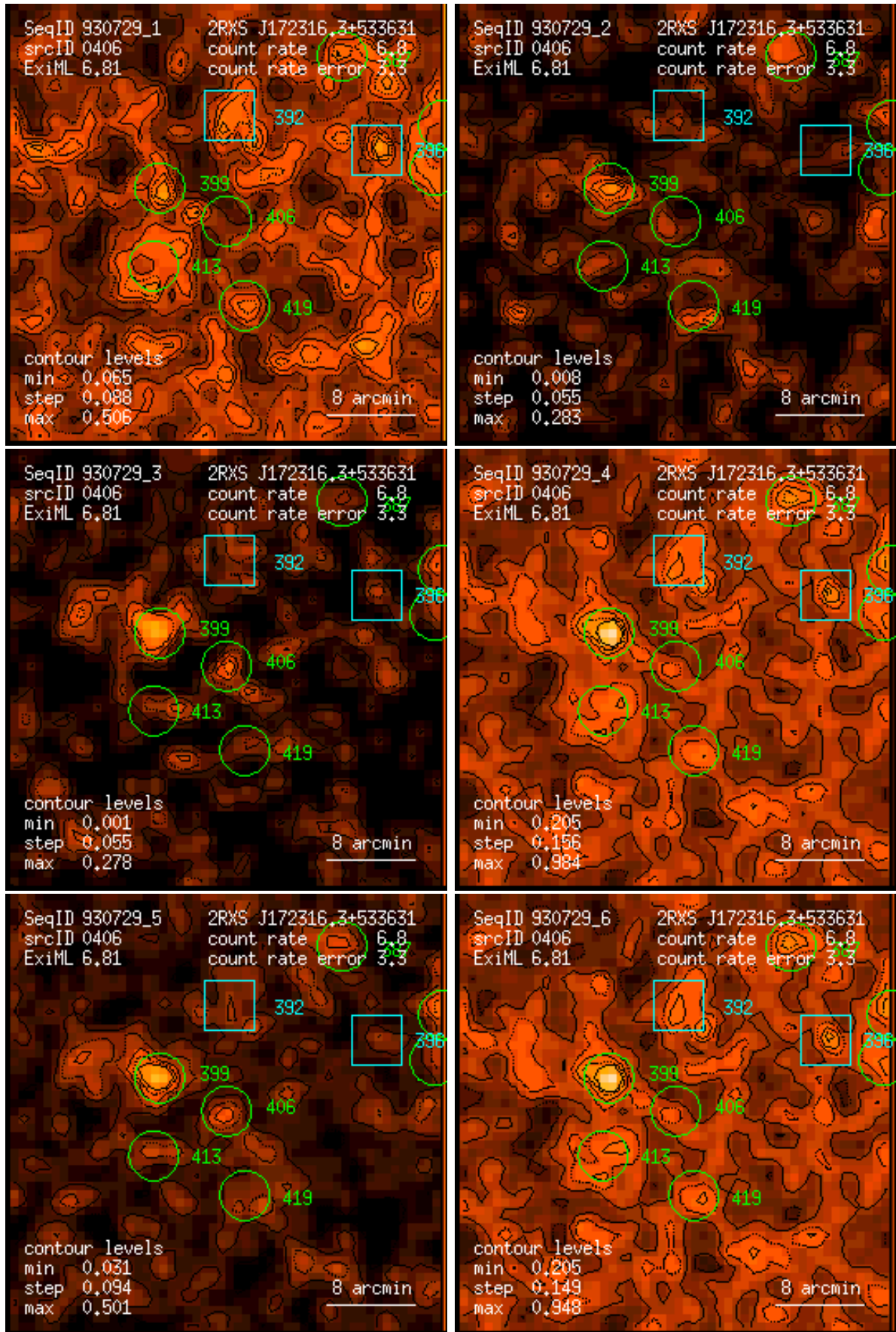
Figure 406: RASS 930729: detection 0406: band rate images, Gaussian filter: (1) PSPC channels 11 – 41, (2) 52 – 90, (3) 91 – 201, (4) 11 – 235, (5) 52 – 201, (6) 11 – 201. Broad band rates in counts/ks. Band rate contour levels in counts/ks/arcmin 2 .
