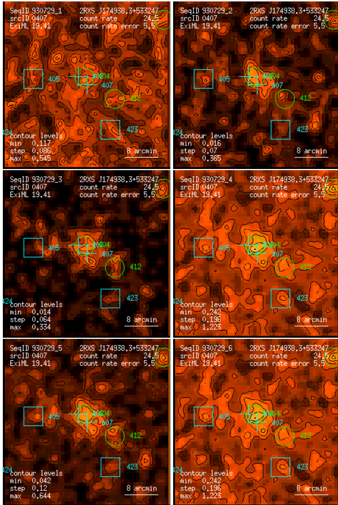
Figure 407: RASS 930729: detection 0407: band rate images, Gaussian filter: (1) PSPC channels 11 – 41, (2) 52 – 90, (3) 91 – 201, (4) 11 – 235, (5) 52 – 201, (6) 11 – 201. Broad band rates in counts/ks. Band rate contour levels in counts/ks/arcmin 2 .
