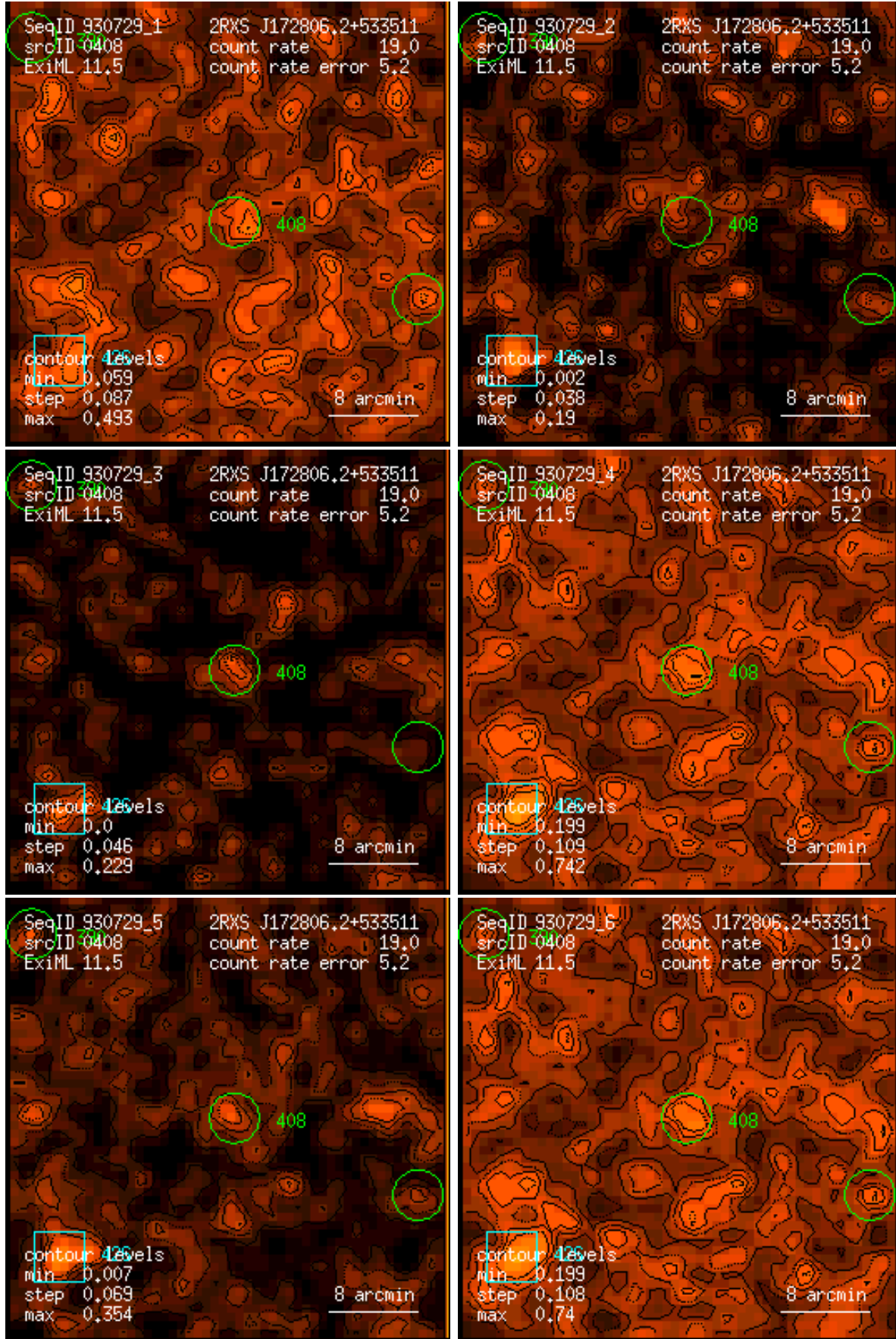
Figure 408: RASS 930729: detection 0408: band rate images, Gaussian filter: (1) PSPC channels 11 – 41, (2) 52 – 90, (3) 91 – 201, (4) 11 – 235, (5) 52 – 201, (6) 11 – 201. Broad band rates in counts/ks. Band rate contour levels in counts/ks/arcmin 2 .
