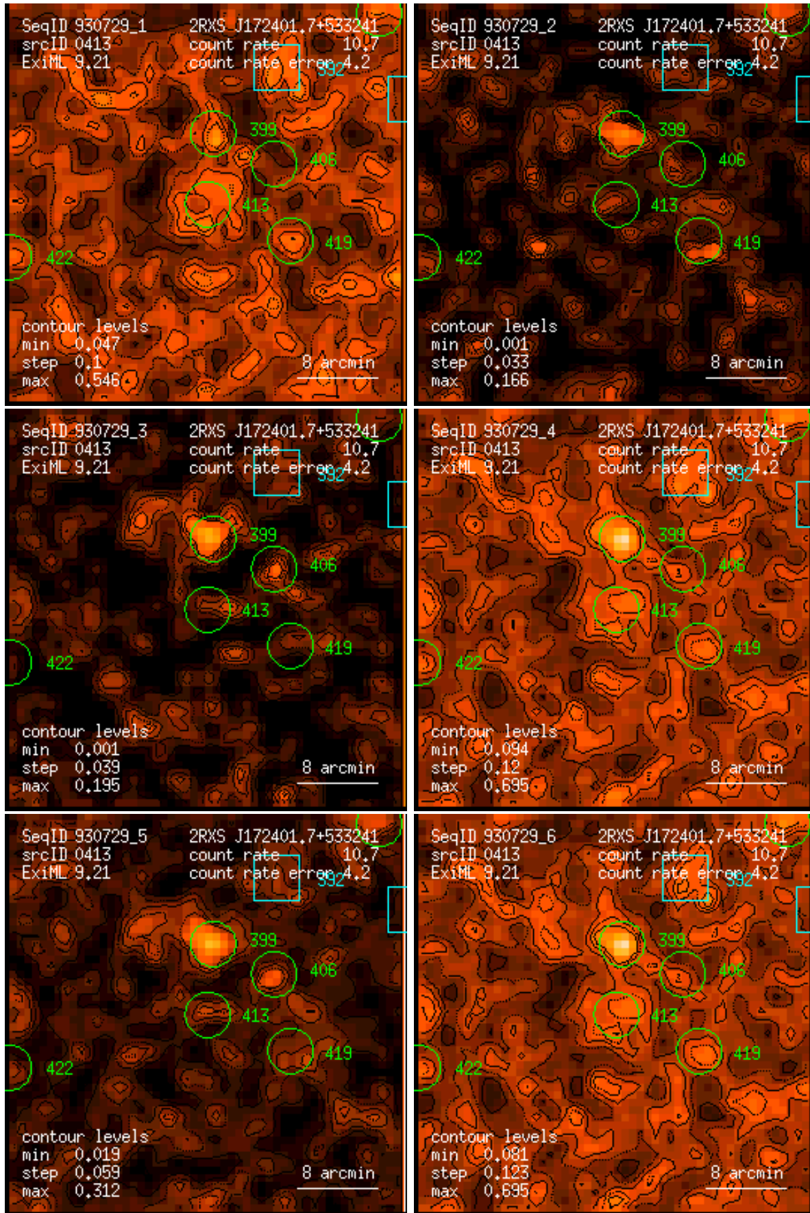
Figure 413: RASS 930729: detection 0413: band rate images, Gaussian filter: (1) PSPC channels 11 – 41, (2) 52 – 90, (3) 91 – 201, (4) 11 – 235, (5) 52 – 201, (6) 11 – 201. Broad band rates in counts/ks. Band rate contour levels in counts/ks/arcmin 2 .
