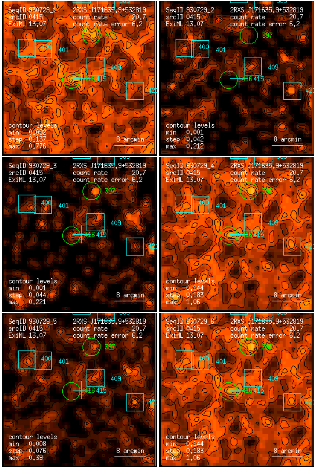
Figure 415: RASS 930729: detection 0415: band rate images, Gaussian filter: (1) PSPC channels 11 – 41, (2) 52 – 90, (3) 91 – 201, (4) 11 – 235, (5) 52 – 201, (6) 11 – 201. Broad band rates in counts/ks. Band rate contour levels in counts/ks/arcmin 2 .
