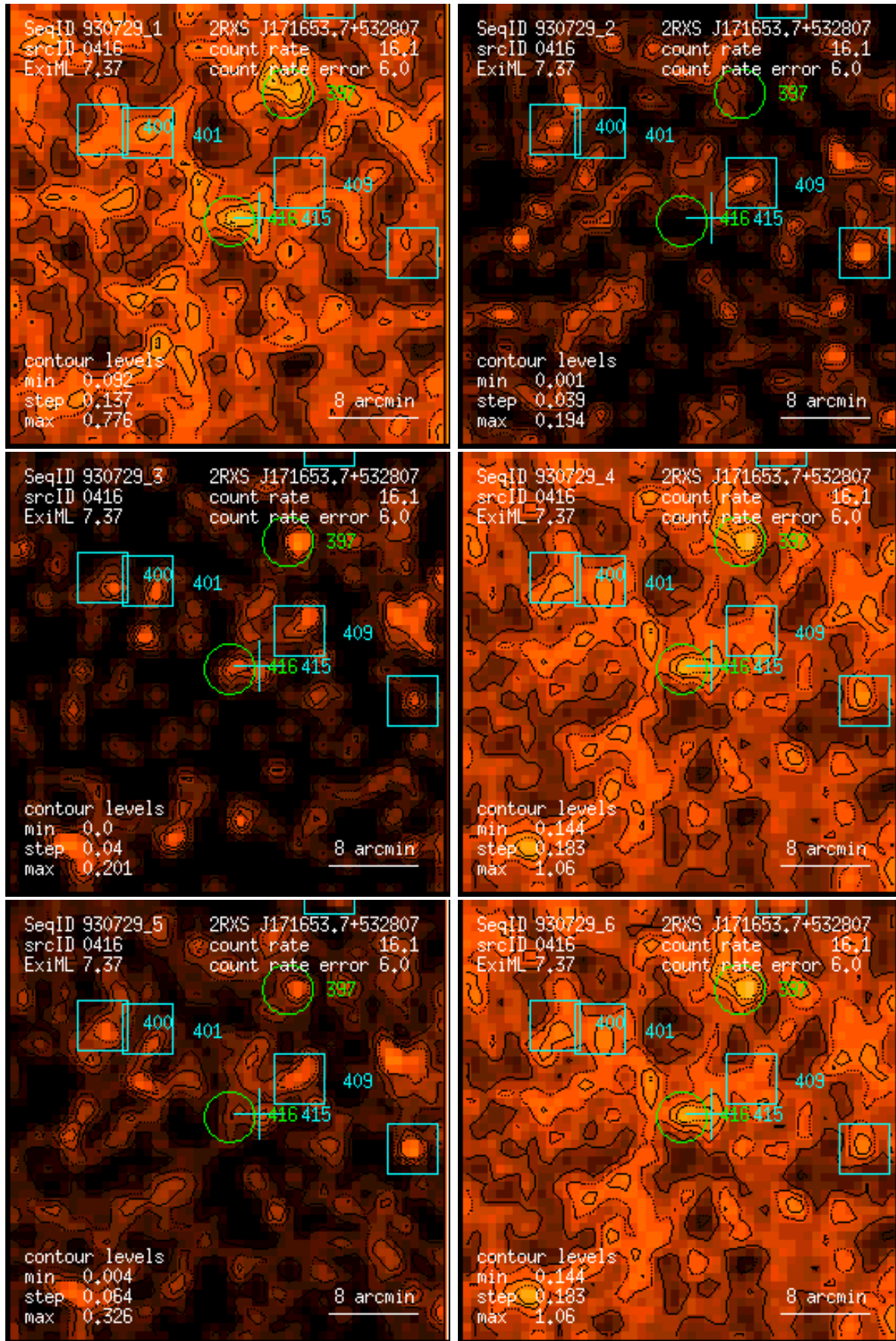
Figure 416: RASS 930729: detection 0416: band rate images, Gaussian filter: (1) PSPC channels 11 – 41, (2) 52 – 90, (3) 91 – 201, (4) 11 – 235, (5) 52 – 201, (6) 11 – 201. Broad band rates in counts/ks. Band rate contour levels in counts/ks/arcmin 2 .
