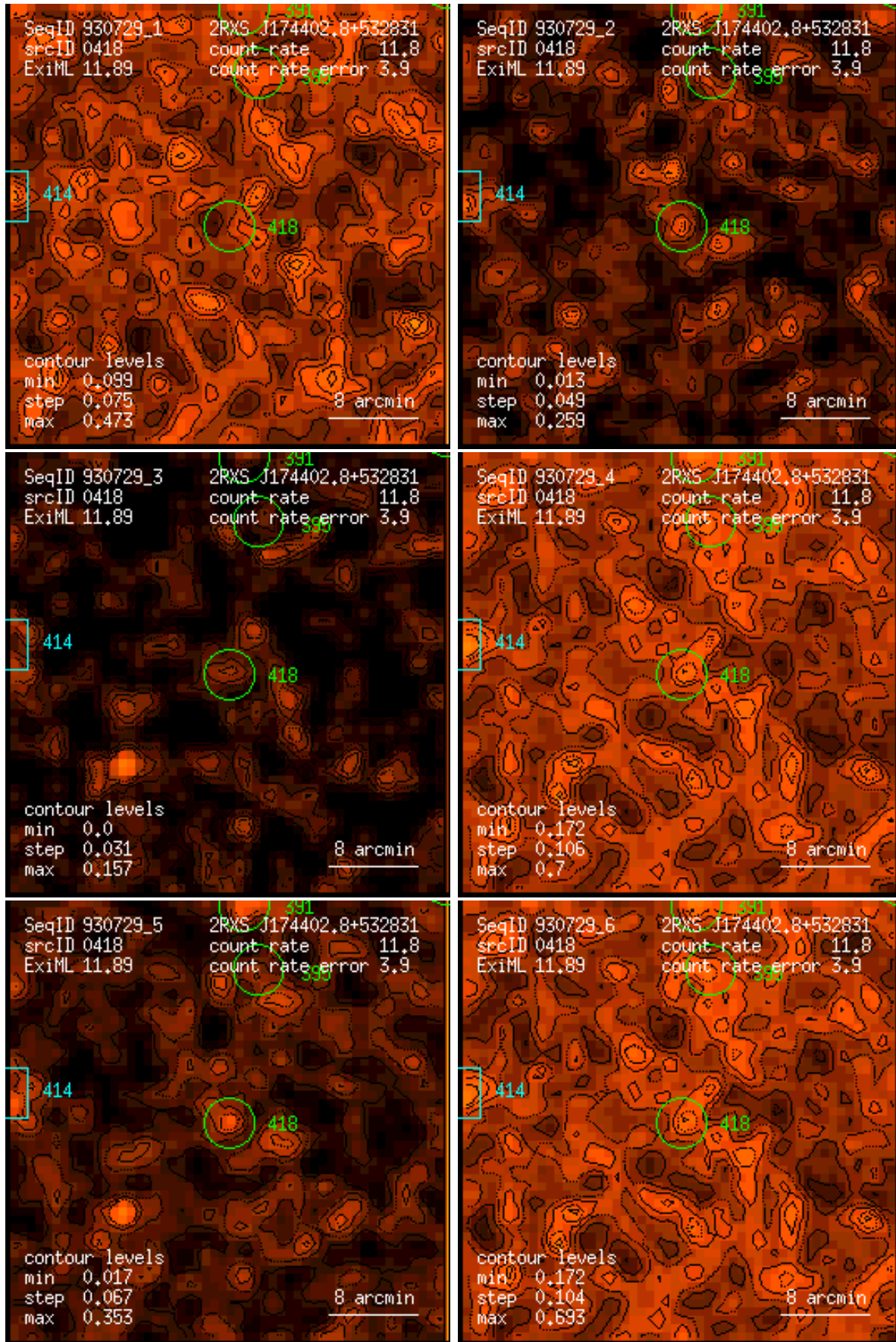
Figure 418: RASS 930729: detection 0418: band rate images, Gaussian filter: (1) PSPC channels 11 – 41, (2) 52 – 90, (3) 91 – 201, (4) 11 – 235, (5) 52 – 201, (6) 11 – 201. Broad band rates in counts/ks. Band rate contour levels in counts/ks/arcmin 2 .
