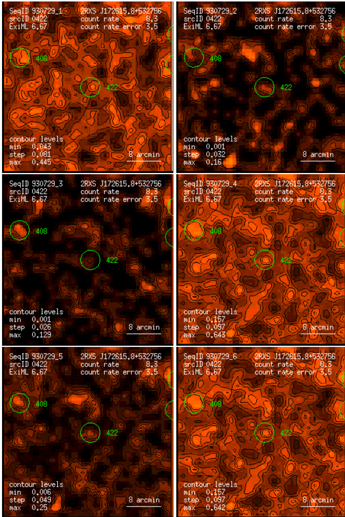
Figure 422: RASS 930729: detection 0422: band rate images, Gaussian filter: (1) PSPC channels 11 – 41, (2) 52 – 90, (3) 91 – 201, (4) 11 – 235, (5) 52 – 201, (6) 11 – 201. Broad band rates in counts/ks. Band rate contour levels in counts/ks/arcmin 2 .
