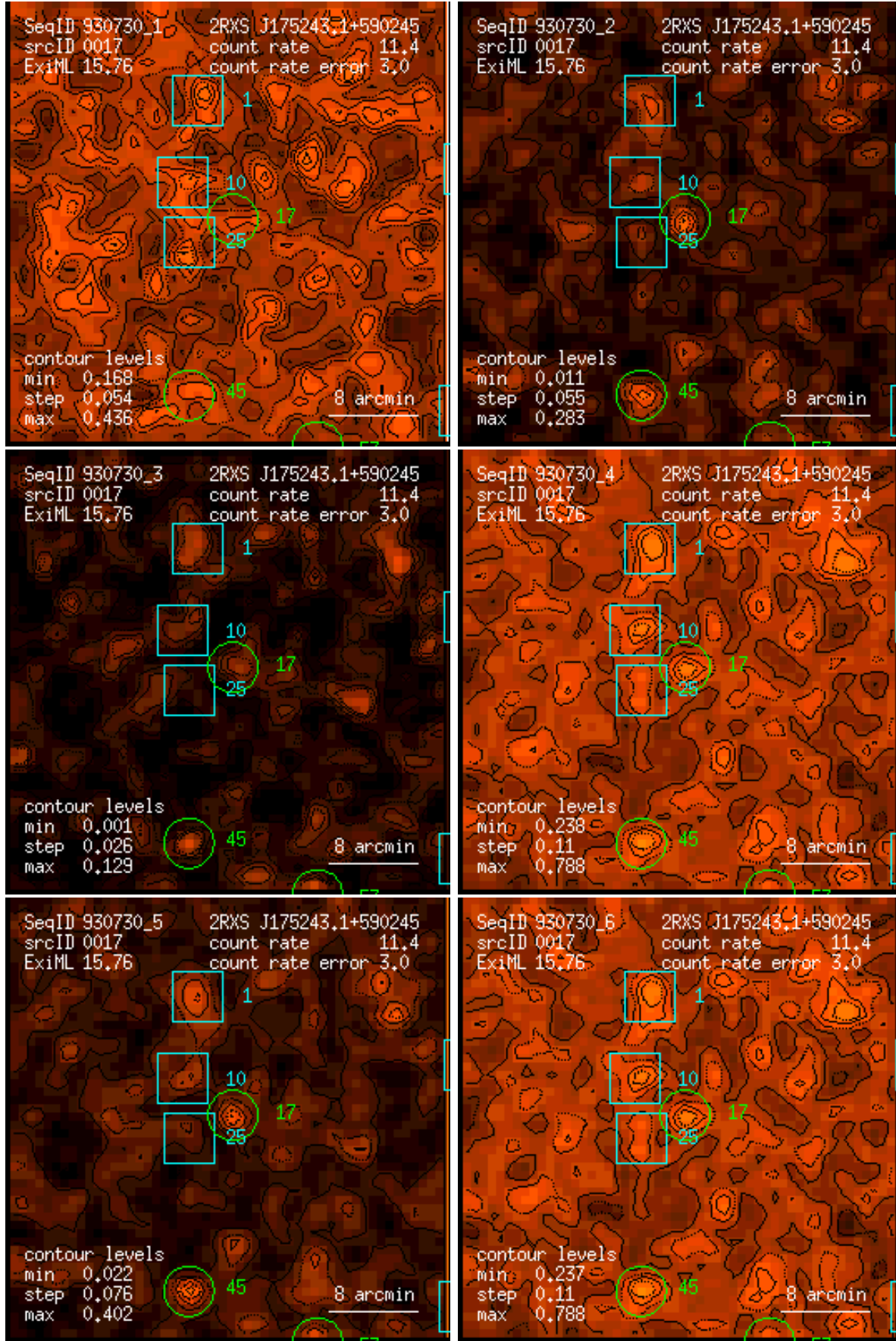
Figure 17: RASS 930730: detection 0017: band rate images, Gaussian filter: (1) PSPC channels 11 – 41, (2) 52 – 90, (3) 91 – 201, (4) 11 – 235, (5) 52 – 201, (6) 11 – 201. Broad band rates in counts/ks. Band rate contour levels in counts/ks/arcmin 2 .
