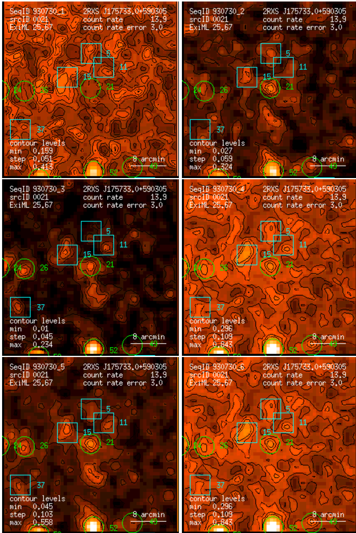
Figure 21: RASS 930730: detection 0021: band rate images, Gaussian filter: (1) PSPC channels 11 – 41, (2) 52 – 90, (3) 91 – 201, (4) 11 – 235, (5) 52 – 201, (6) 11 – 201. Broad band rates in counts/ks. Band rate contour levels in counts/ks/arcmin 2 .
