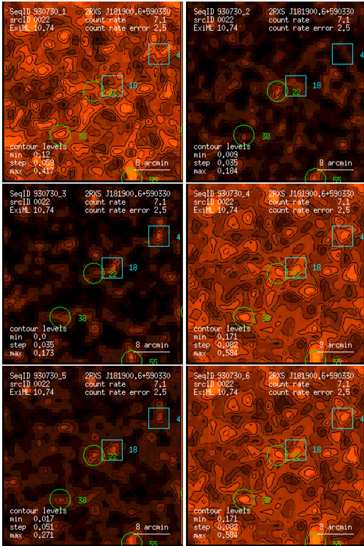
Figure 22: RASS 930730: detection 0022: band rate images, Gaussian filter: (1) PSPC channels 11 – 41, (2) 52 – 90, (3) 91 – 201, (4) 11 – 235, (5) 52 – 201, (6) 11 – 201. Broad band rates in counts/ks. Band rate contour levels in counts/ks/arcmin 2 .
