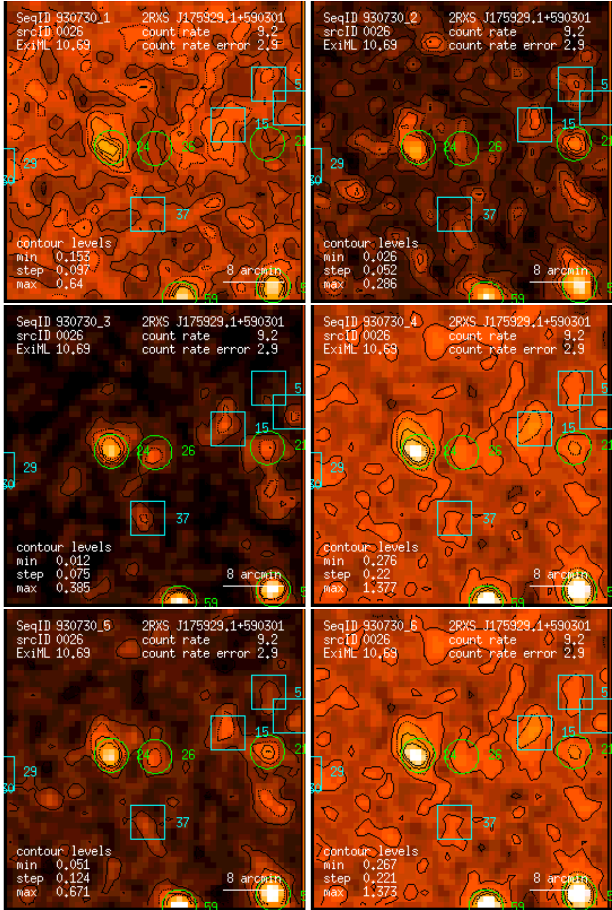
Figure 26: RASS 930730: detection 0026: band rate images, Gaussian filter: (1) PSPC channels 11 – 41, (2) 52 – 90, (3) 91 – 201, (4) 11 – 235, (5) 52 – 201, (6) 11 – 201. Broad band rates in counts/ks. Band rate contour levels in counts/ks/arcmin 2 .
