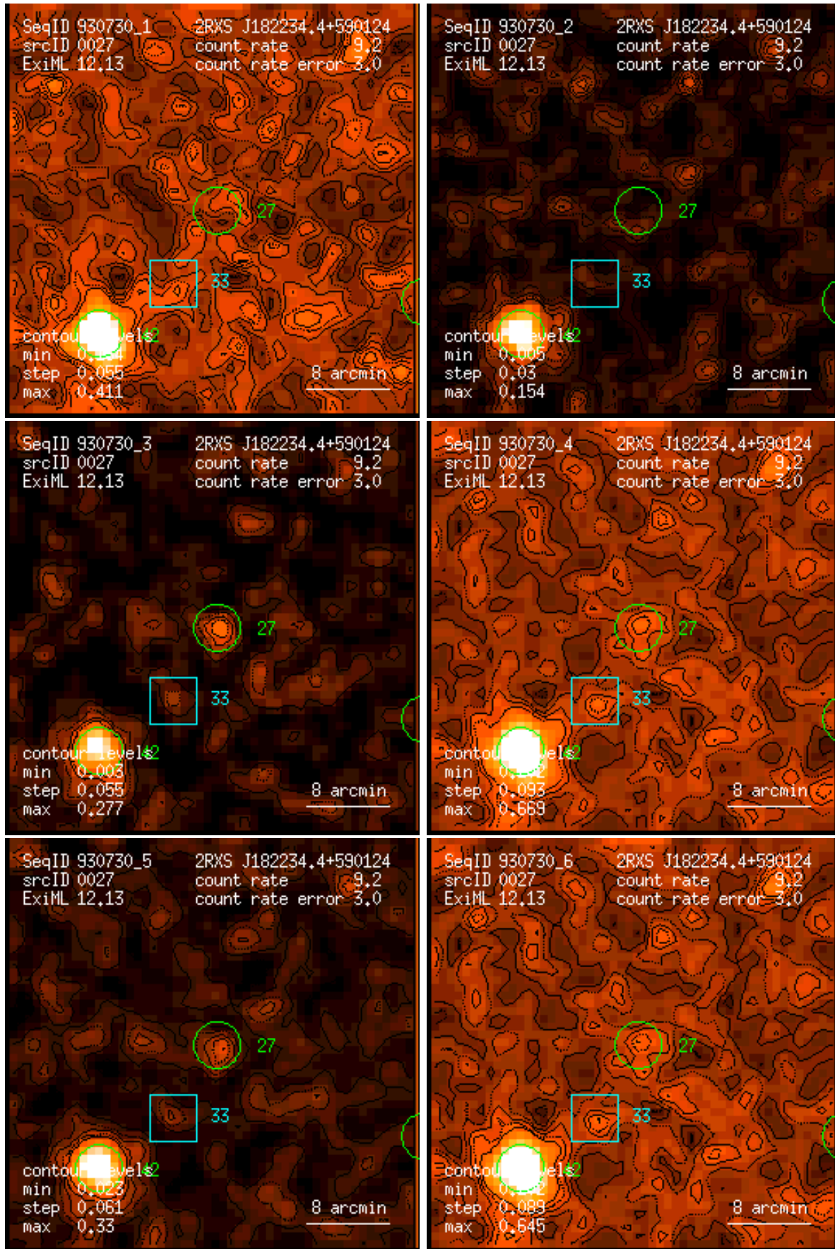
Figure 27: RASS 930730: detection 0027: band rate images, Gaussian filter: (1) PSPC channels 11 – 41, (2) 52 – 90, (3) 91 – 201, (4) 11 – 235, (5) 52 – 201, (6) 11 – 201. Broad band rates in counts/ks. Band rate contour levels in counts/ks/arcmin 2 .
