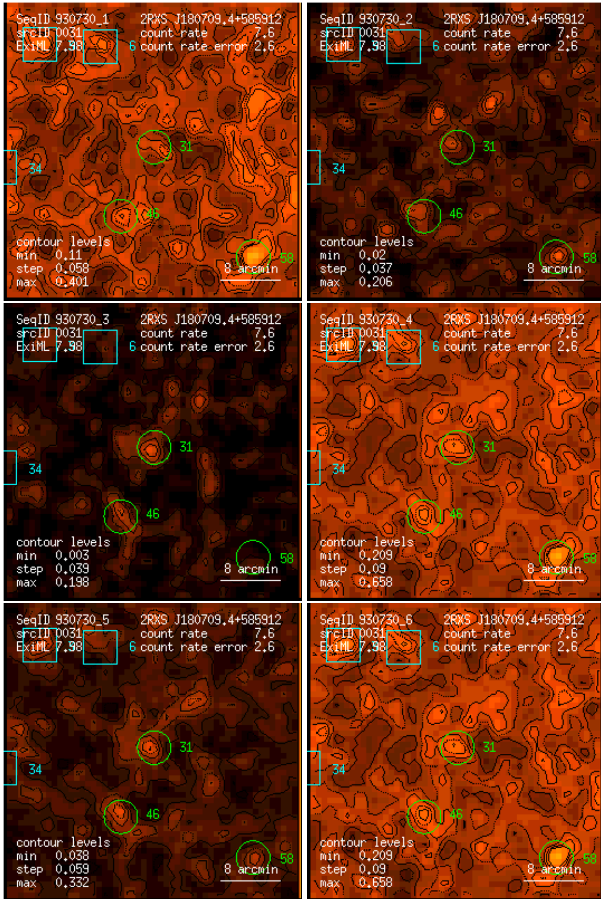
Figure 31: RASS 930730: detection 0031: band rate images, Gaussian filter: (1) PSPC channels 11 – 41, (2) 52 – 90, (3) 91 – 201, (4) 11 – 235, (5) 52 – 201, (6) 11 – 201. Broad band rates in counts/ks. Band rate contour levels in counts/ks/arcmin 2 .
