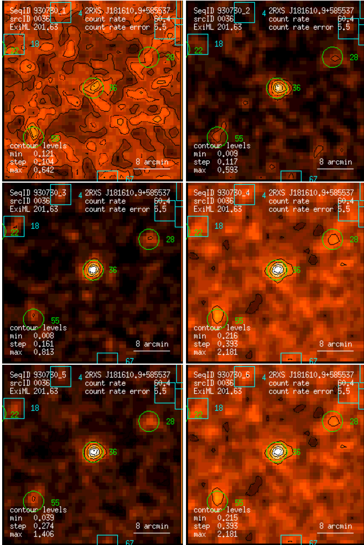
Figure 36: RASS 930730: detection 0036: band rate images, Gaussian filter: (1) PSPC channels 11 – 41, (2) 52 – 90, (3) 91 – 201, (4) 11 – 235, (5) 52 – 201, (6) 11 – 201. Broad band rates in counts/ks. Band rate contour levels in counts/ks/arcmin 2 .
