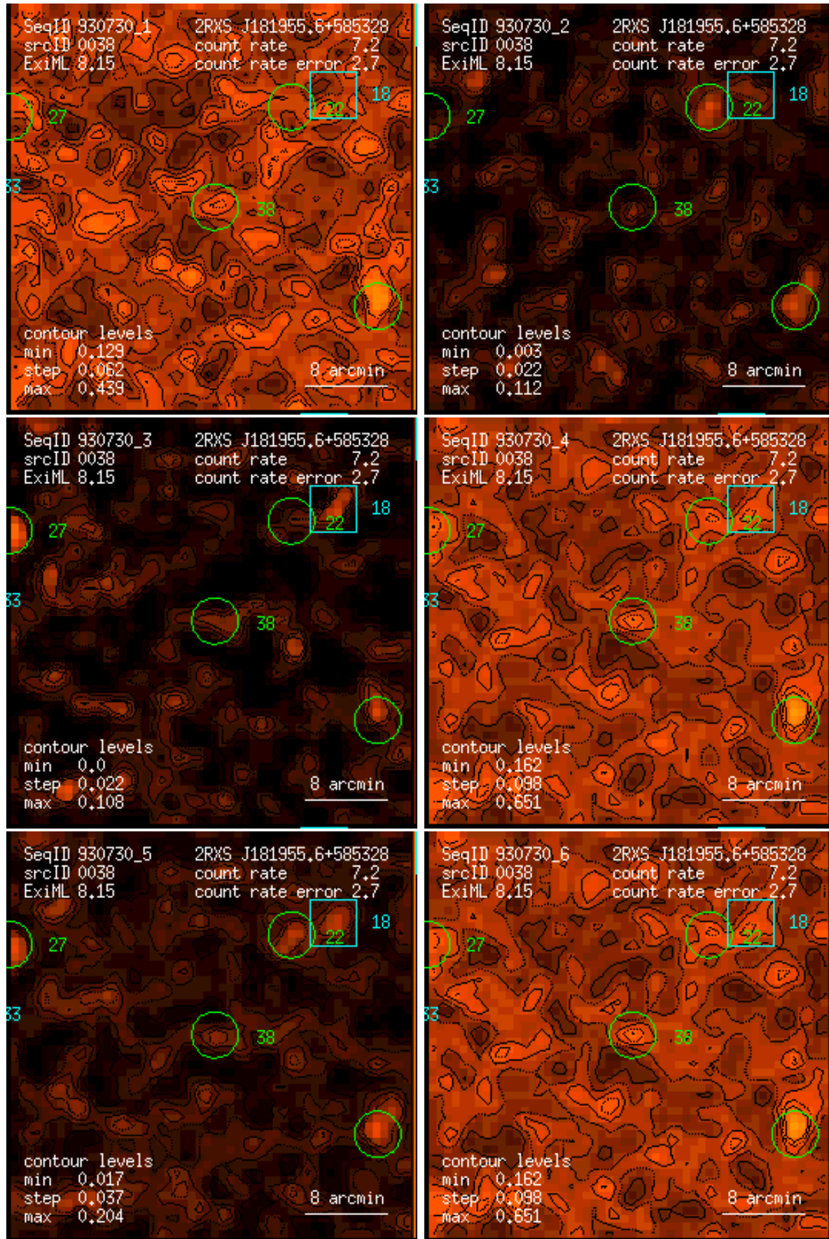
Figure 38: RASS 930730: detection 0038: band rate images, Gaussian filter: (1) PSPC channels 11 – 41, (2) 52 – 90, (3) 91 – 201, (4) 11 – 235, (5) 52 – 201, (6) 11 – 201. Broad band rates in counts/ks. Band rate contour levels in counts/ks/arcmin 2 .
