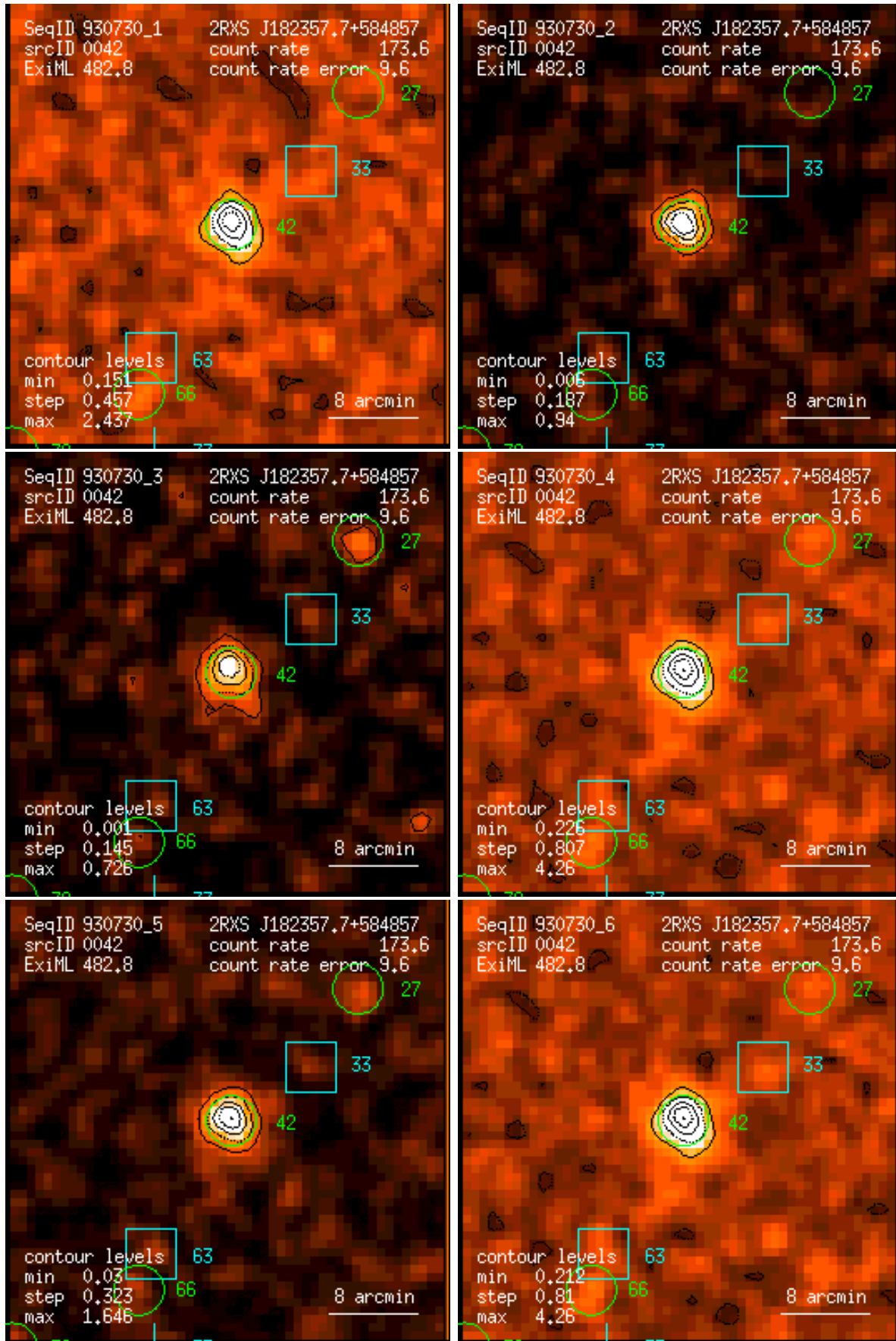
Figure 42: RASS 930730: detection 0042: band rate images, Gaussian filter: (1) PSPC channels 11 – 41, (2) 52 – 90, (3) 91 – 201, (4) 11 – 235, (5) 52 – 201, (6) 11 – 201. Broad band rates in counts/ks. Band rate contour levels in counts/ks/arcmin 2 .
