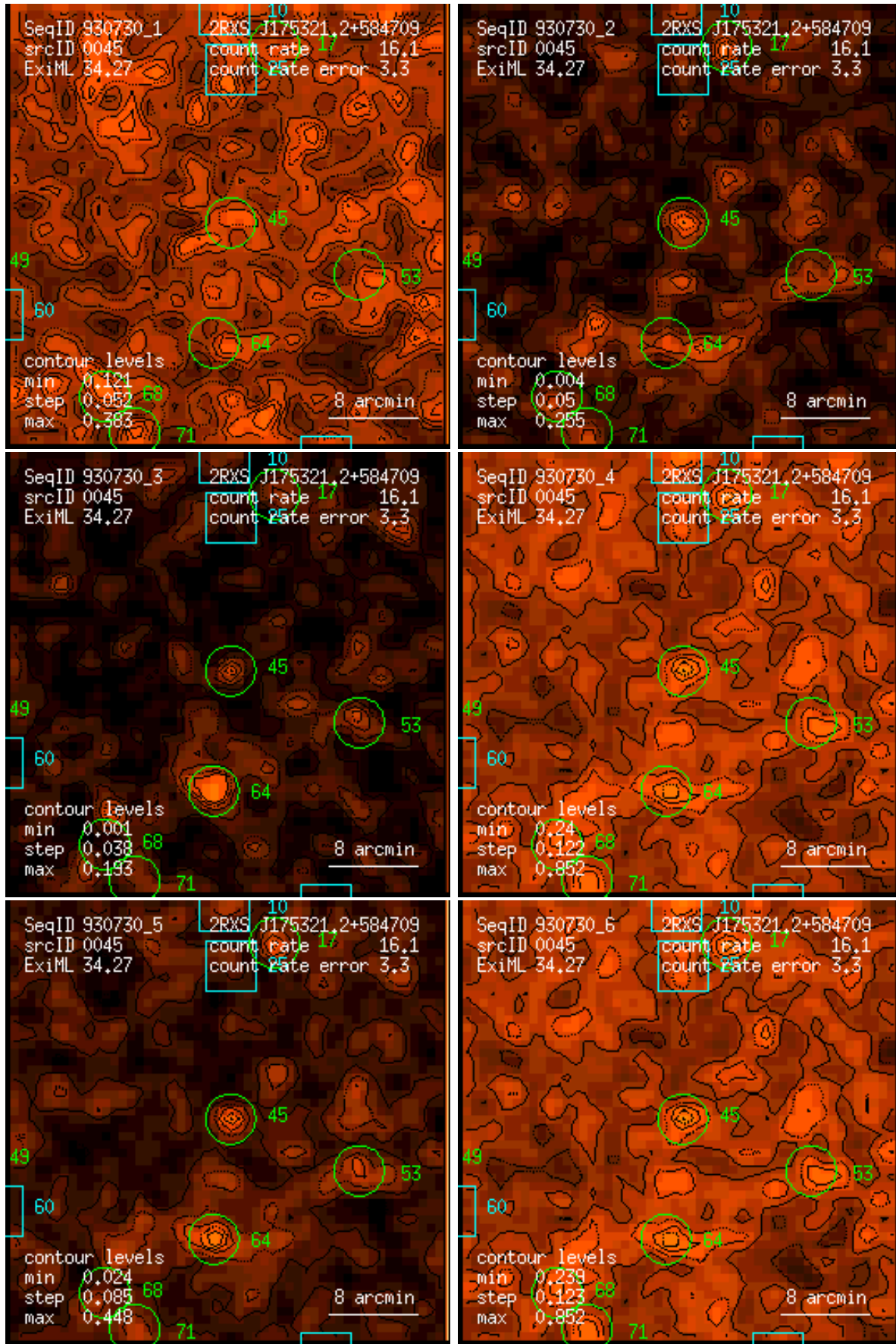
Figure 45: RASS 930730: detection 0045: band rate images, Gaussian filter: (1) PSPC channels 11 – 41, (2) 52 – 90, (3) 91 – 201, (4) 11 – 235, (5) 52 – 201, (6) 11 – 201. Broad band rates in counts/ks. Band rate contour levels in counts/ks/arcmin 2 .
