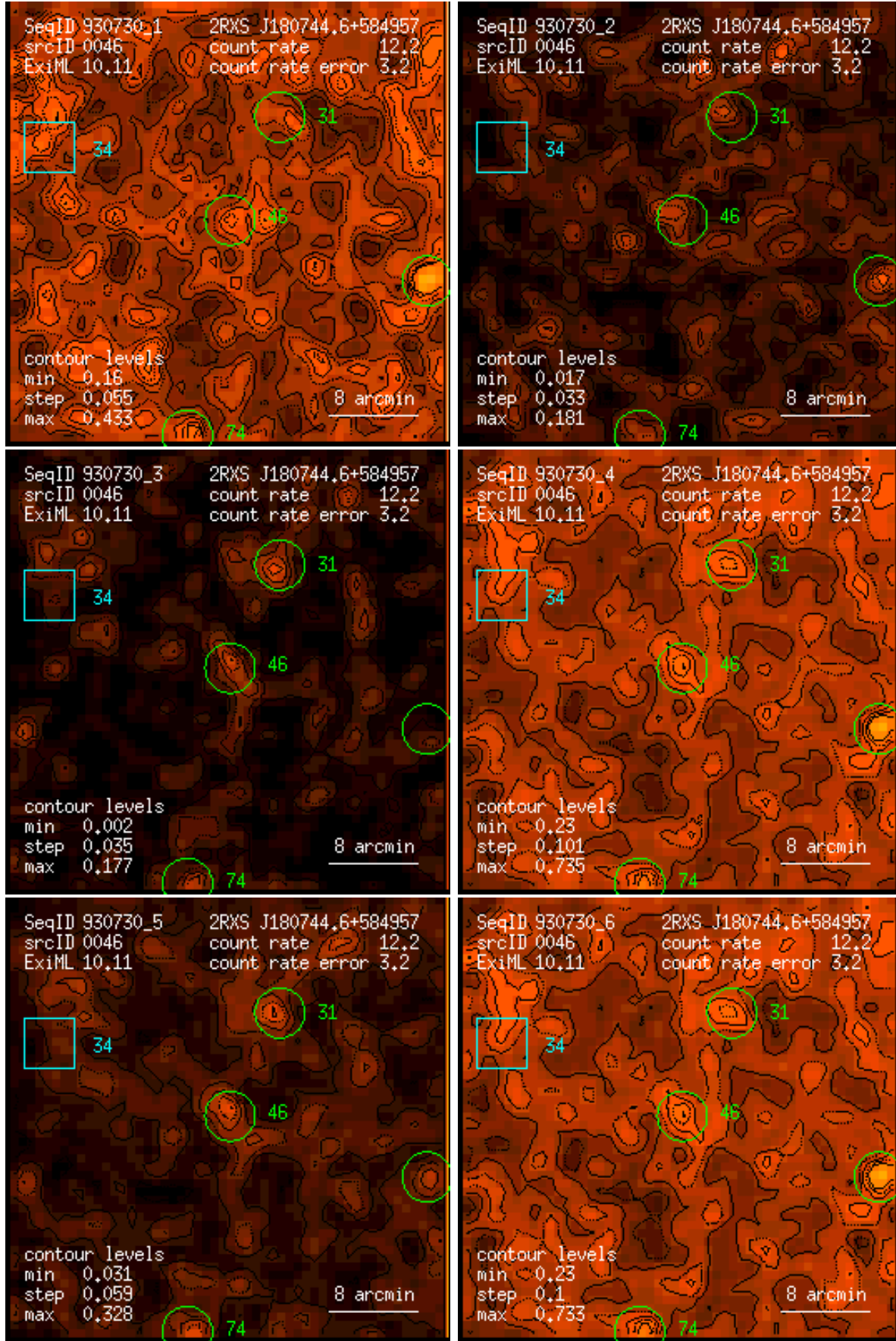
Figure 46: RASS 930730: detection 0046: band rate images, Gaussian filter: (1) PSPC channels 11 – 41, (2) 52 – 90, (3) 91 – 201, (4) 11 – 235, (5) 52 – 201, (6) 11 – 201. Broad band rates in counts/ks. Band rate contour levels in counts/ks/arcmin 2 .
