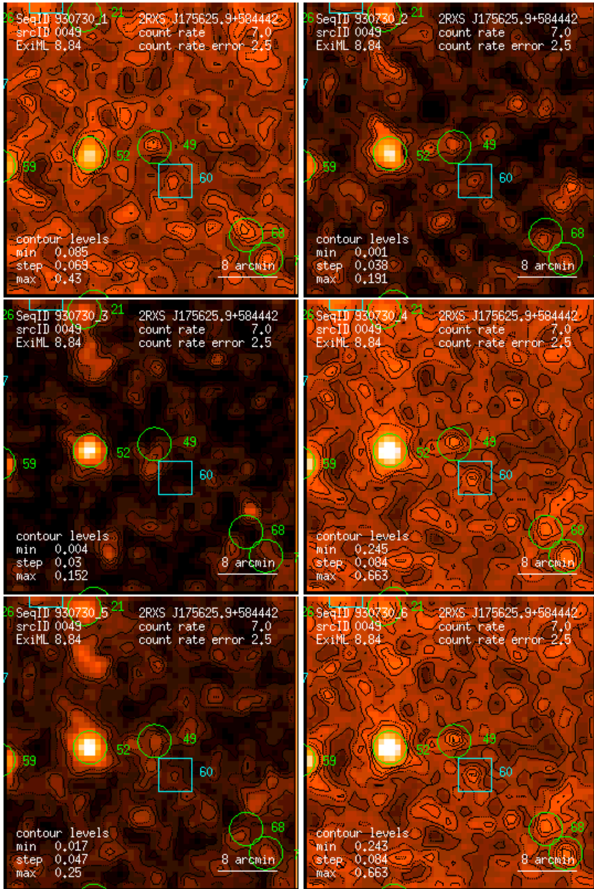
Figure 49: RASS 930730: detection 0049: band rate images, Gaussian filter: (1) PSPC channels 11 – 41, (2) 52 – 90, (3) 91 – 201, (4) 11 – 235, (5) 52 – 201, (6) 11 – 201. Broad band rates in counts/ks. Band rate contour levels in counts/ks/arcmin 2 .
