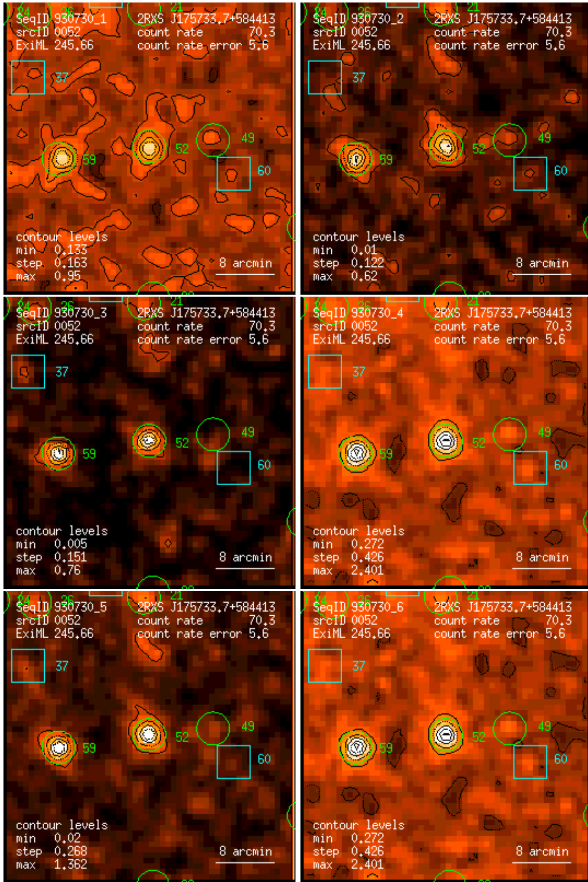
Figure 52: RASS 930730: detection 0052: band rate images, Gaussian filter: (1) PSPC channels 11 – 41, (2) 52 – 90, (3) 91 – 201, (4) 11 – 235, (5) 52 – 201, (6) 11 – 201. Broad band rates in counts/ks. Band rate contour levels in counts/ks/arcmin 2 .
