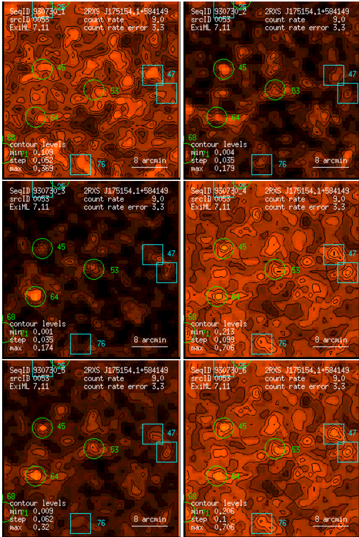
Figure 53: RASS 930730: detection 0053: band rate images, Gaussian filter: (1) PSPC channels 11 – 41, (2) 52 – 90, (3) 91 – 201, (4) 11 – 235, (5) 52 – 201, (6) 11 – 201. Broad band rates in counts/ks. Band rate contour levels in counts/ks/arcmin 2 .
