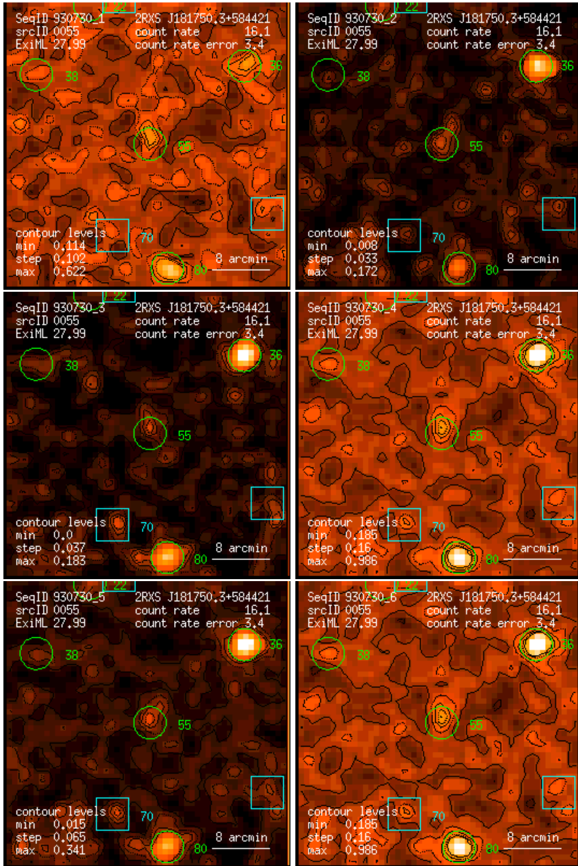
Figure 55: RASS 930730: detection 0055: band rate images, Gaussian filter: (1) PSPC channels 11 – 41, (2) 52 – 90, (3) 91 – 201, (4) 11 – 235, (5) 52 – 201, (6) 11 – 201. Broad band rates in counts/ks. Band rate contour levels in counts/ks/arcmin 2 .
