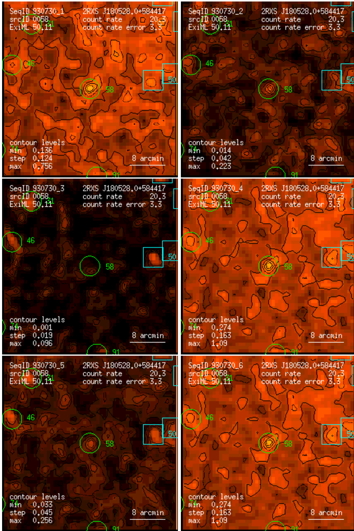
Figure 58: RASS 930730: detection 0058: band rate images, Gaussian filter: (1) PSPC channels 11 – 41, (2) 52 – 90, (3) 91 – 201, (4) 11 – 235, (5) 52 – 201, (6) 11 – 201. Broad band rates in counts/ks. Band rate contour levels in counts/ks/arcmin 2 .
