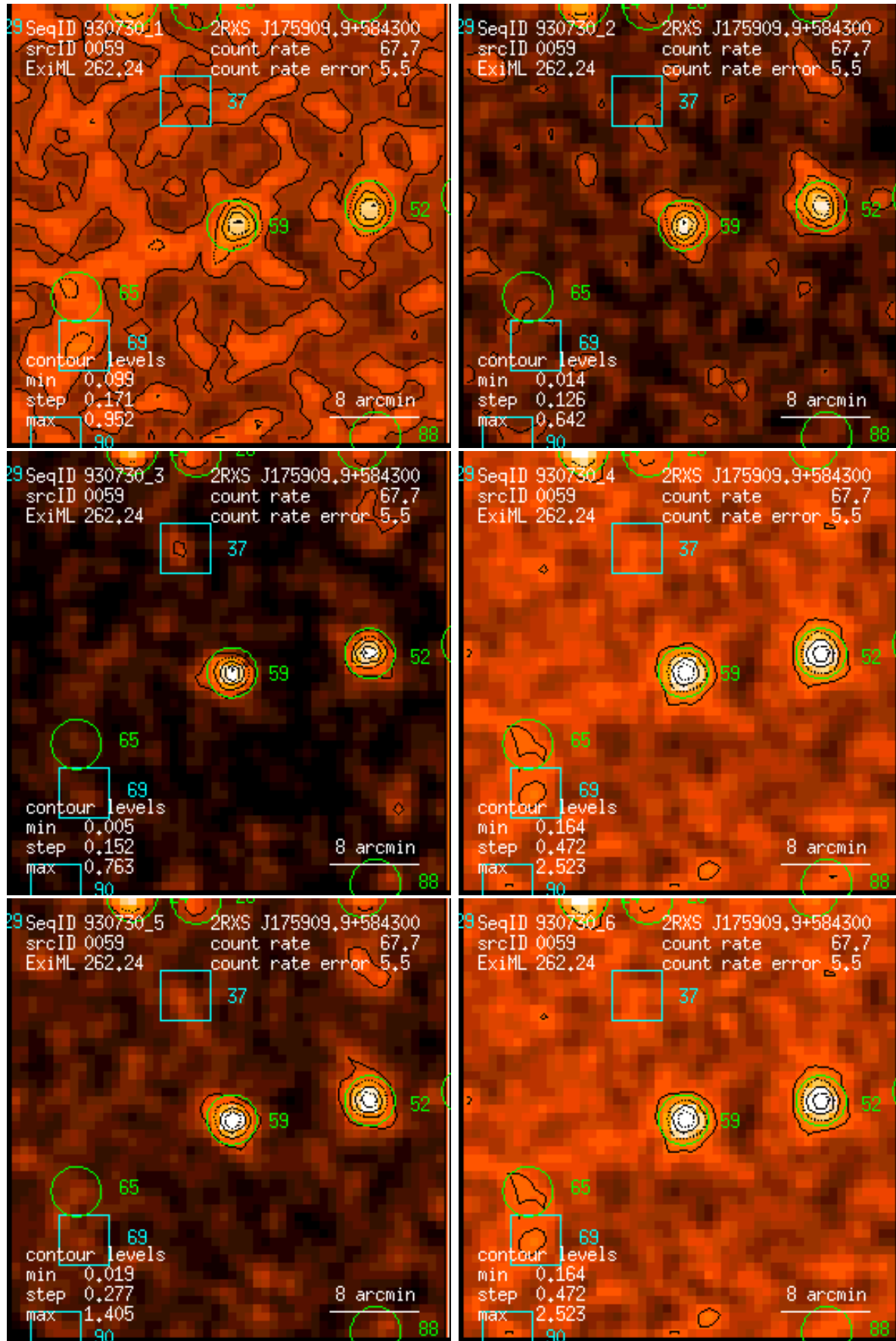
Figure 59: RASS 930730: detection 0059: band rate images, Gaussian filter: (1) PSPC channels 11 – 41, (2) 52 – 90, (3) 91 – 201, (4) 11 – 235, (5) 52 – 201, (6) 11 – 201. Broad band rates in counts/ks. Band rate contour levels in counts/ks/arcmin 2 .
