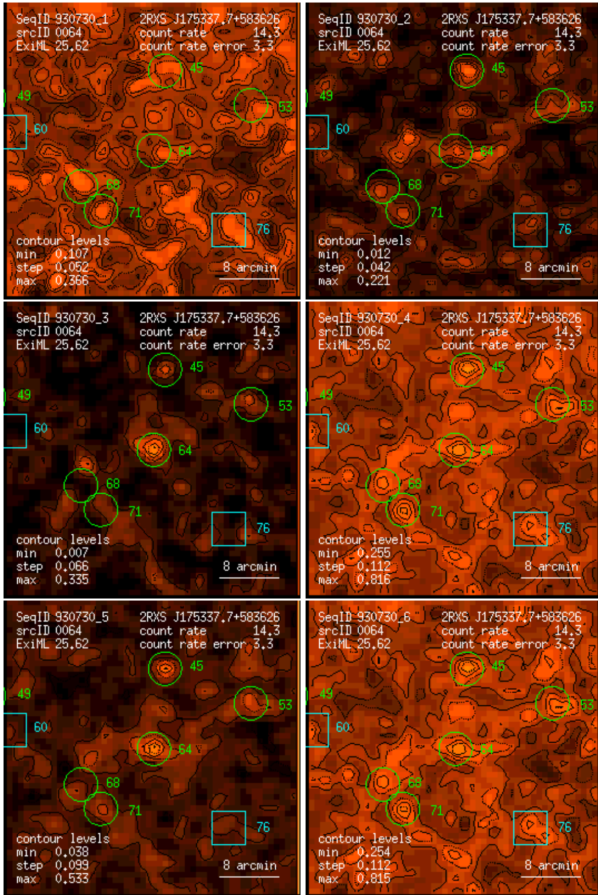
Figure 64: RASS 930730: detection 0064: band rate images, Gaussian filter: (1) PSPC channels 11 – 41, (2) 52 – 90, (3) 91 – 201, (4) 11 – 235, (5) 52 – 201, (6) 11 – 201. Broad band rates in counts/ks. Band rate contour levels in counts/ks/arcmin 2 .
