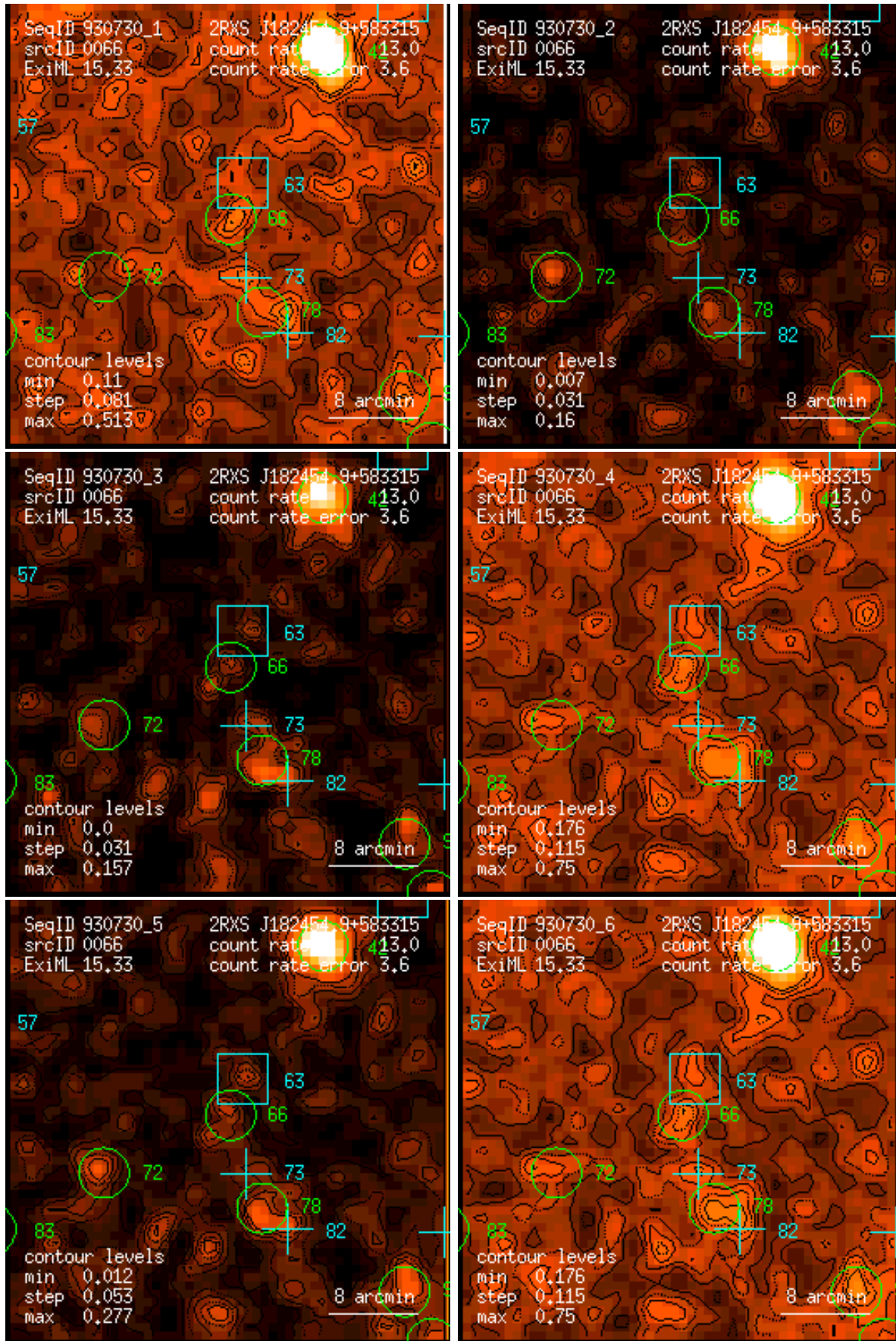
Figure 66: RASS 930730: detection 0066: band rate images, Gaussian filter: (1) PSPC channels 11 – 41, (2) 52 – 90, (3) 91 – 201, (4) 11 – 235, (5) 52 – 201, (6) 11 – 201. Broad band rates in counts/ks. Band rate contour levels in counts/ks/arcmin 2 .
