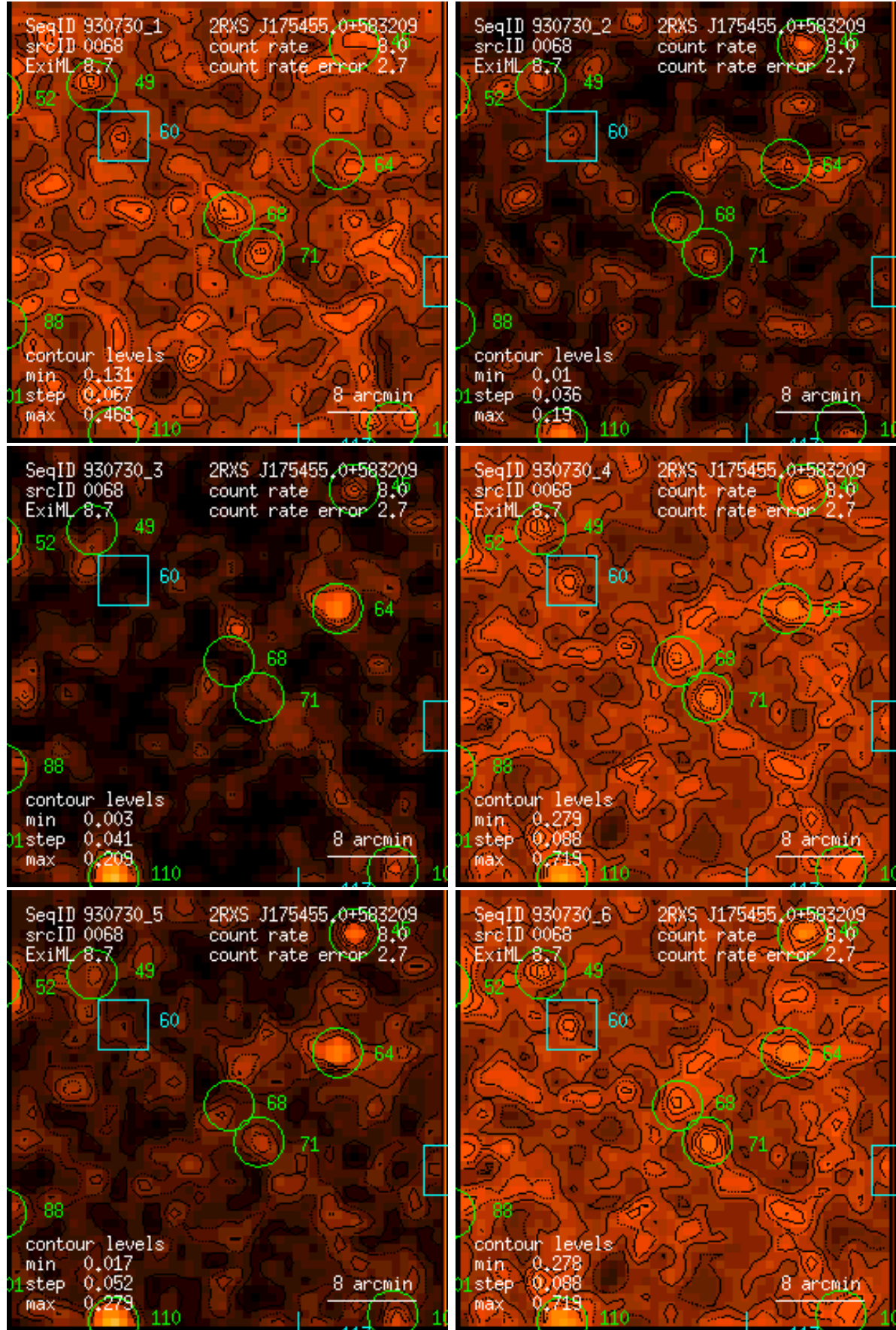
Figure 68: RASS 930730: detection 0068: band rate images, Gaussian filter: (1) PSPC channels 11 – 41, (2) 52 – 90, (3) 91 – 201, (4) 11 – 235, (5) 52 – 201, (6) 11 – 201. Broad band rates in counts/ks. Band rate contour levels in counts/ks/arcmin 2 .
