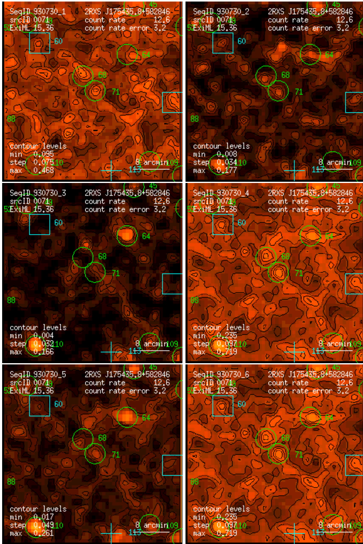
Figure 71: RASS 930730: detection 0071: band rate images, Gaussian filter: (1) PSPC channels 11 – 41, (2) 52 – 90, (3) 91 – 201, (4) 11 – 235, (5) 52 – 201, (6) 11 – 201. Broad band rates in counts/ks. Band rate contour levels in counts/ks/arcmin 2 .
