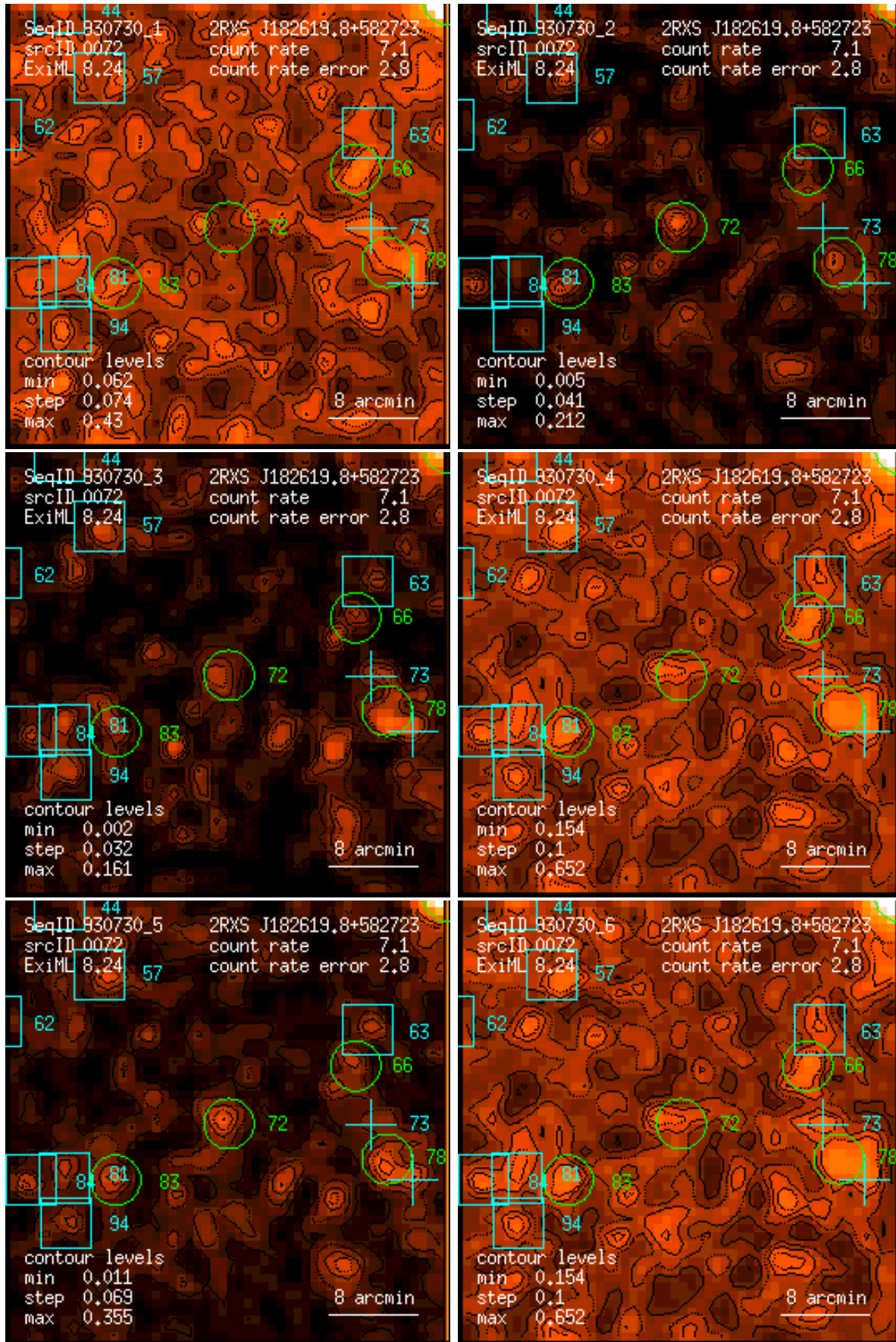
Figure 72: RASS 930730: detection 0072: band rate images, Gaussian filter: (1) PSPC channels 11 – 41, (2) 52 – 90, (3) 91 – 201, (4) 11 – 235, (5) 52 – 201, (6) 11 – 201. Broad band rates in counts/ks. Band rate contour levels in counts/ks/arcmin 2 .
