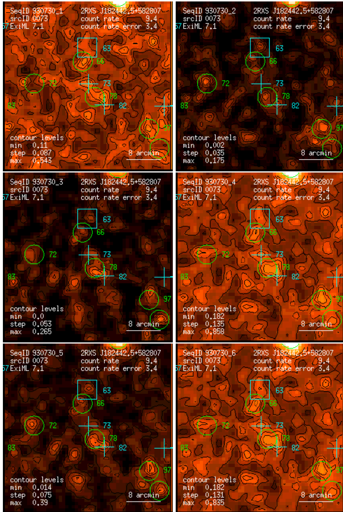
Figure 73: RASS 930730: detection 0073: band rate images, Gaussian filter: (1) PSPC channels 11 – 41, (2) 52 – 90, (3) 91 – 201, (4) 11 – 235, (5) 52 – 201, (6) 11 – 201. Broad band rates in counts/ks. Band rate contour levels in counts/ks/arcmin 2 .
