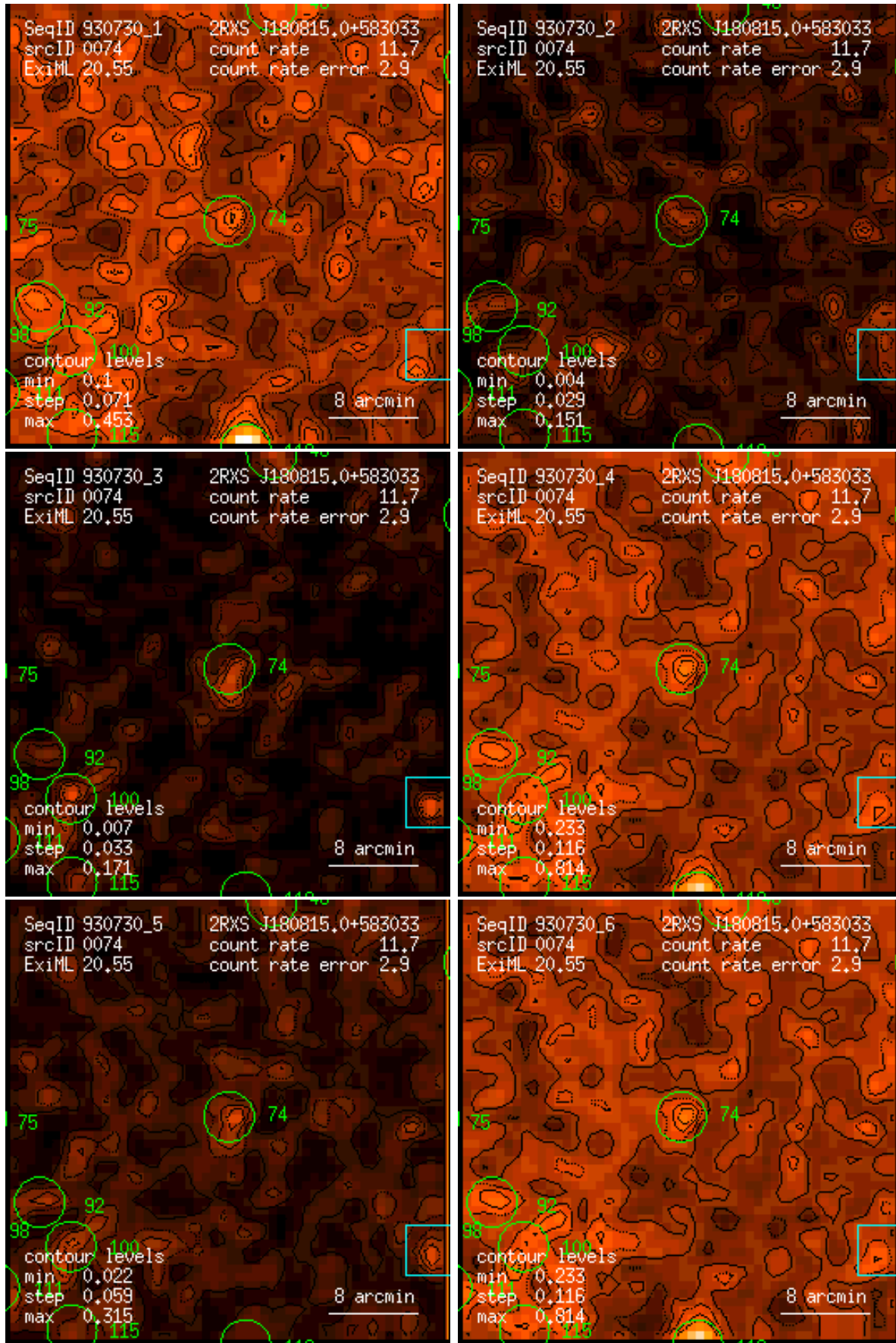
Figure 74: RASS 930730: detection 0074: band rate images, Gaussian filter: (1) PSPC channels 11 – 41, (2) 52 – 90, (3) 91 – 201, (4) 11 – 235, (5) 52 – 201, (6) 11 – 201. Broad band rates in counts/ks. Band rate contour levels in counts/ks/arcmin 2 .
