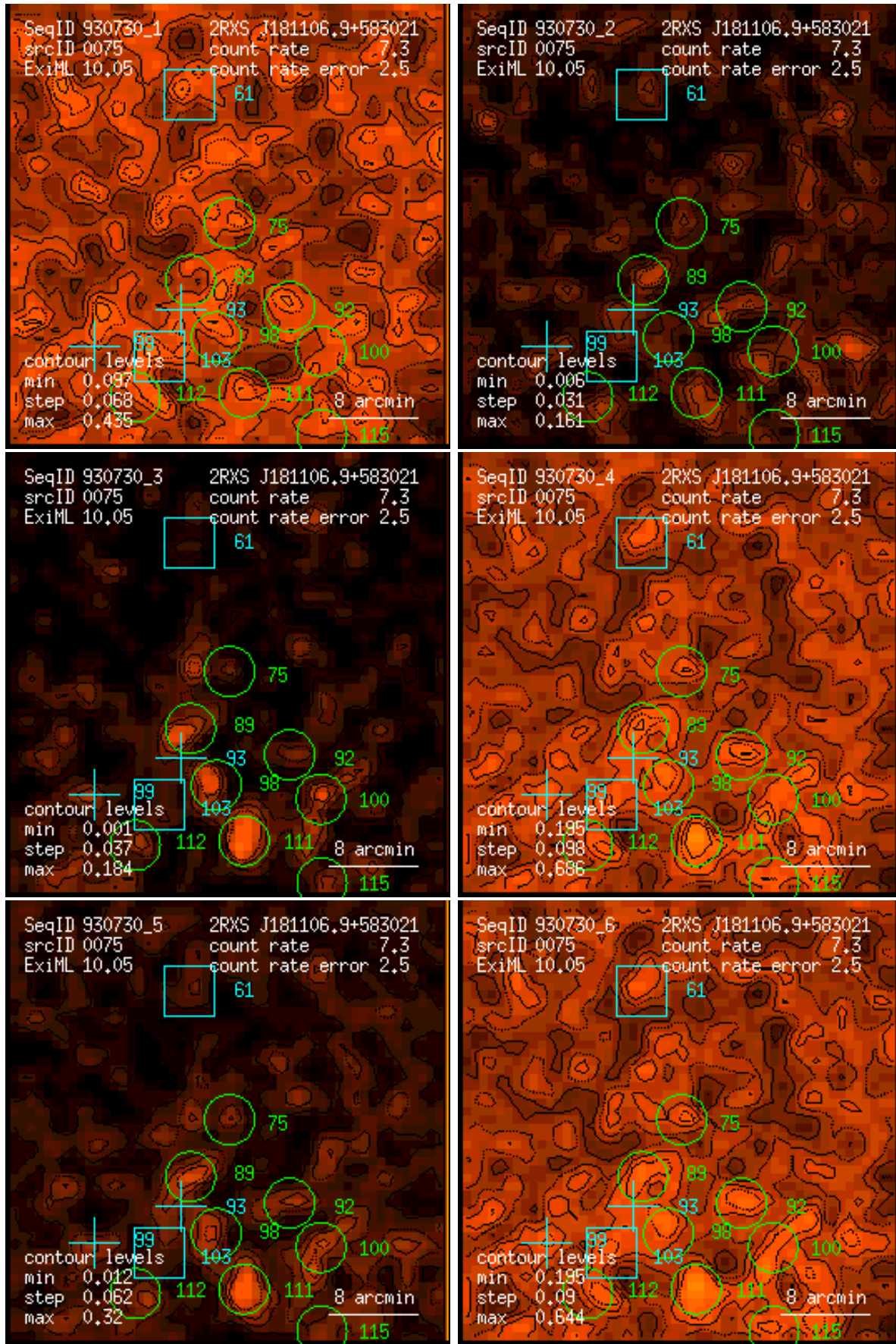
Figure 75: RASS 930730: detection 0075: band rate images, Gaussian filter: (1) PSPC channels 11 – 41, (2) 52 – 90, (3) 91 – 201, (4) 11 – 235, (5) 52 – 201, (6) 11 – 201. Broad band rates in counts/ks. Band rate contour levels in counts/ks/arcmin 2 .
