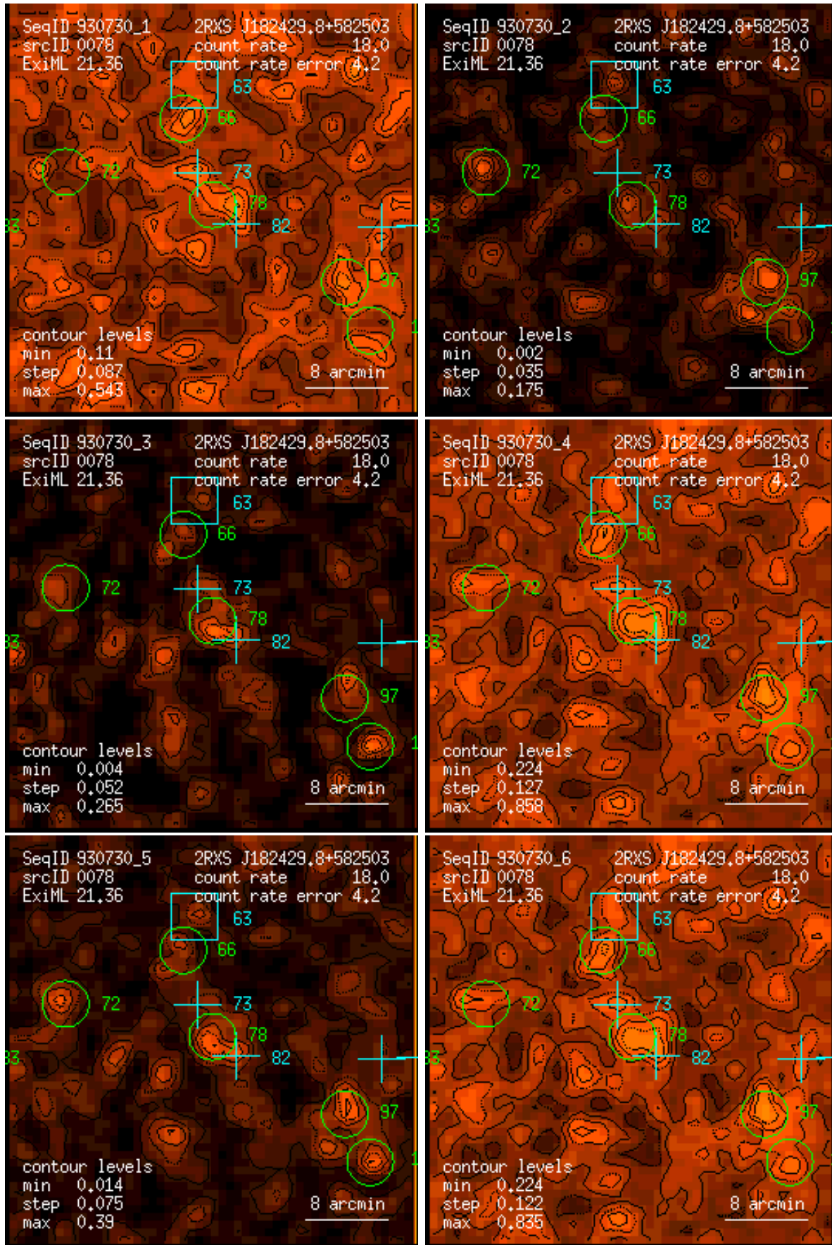
Figure 78: RASS 930730: detection 0078: band rate images, Gaussian filter: (1) PSPC channels 11 – 41, (2) 52 – 90, (3) 91 – 201, (4) 11 – 235, (5) 52 – 201, (6) 11 – 201. Broad band rates in counts/ks. Band rate contour levels in counts/ks/arcmin 2 .
