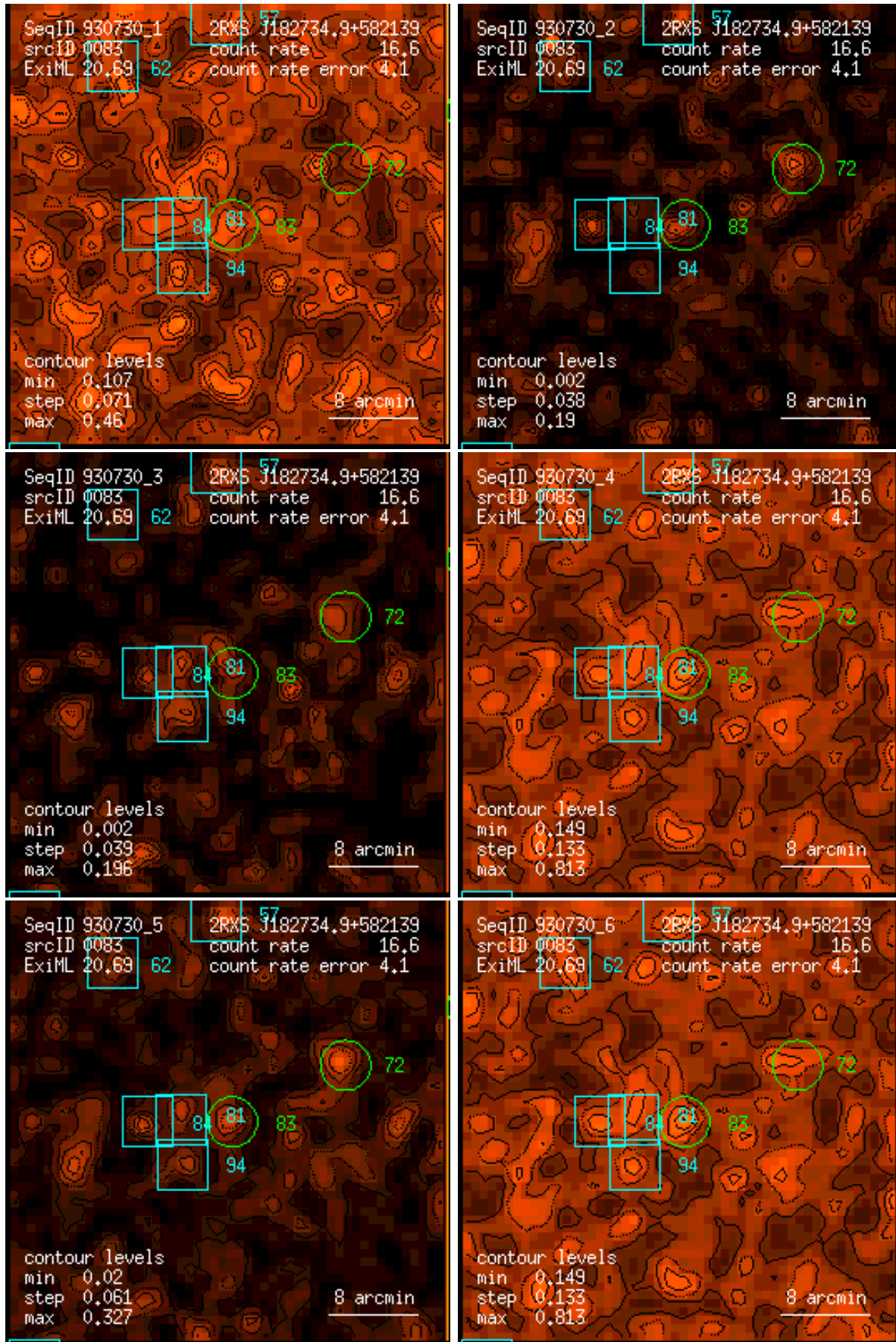
Figure 83: RASS 930730: detection 0083: band rate images, Gaussian filter: (1) PSPC channels 11 – 41, (2) 52 – 90, (3) 91 – 201, (4) 11 – 235, (5) 52 – 201, (6) 11 – 201. Broad band rates in counts/ks. Band rate contour levels in counts/ks/arcmin 2 .
