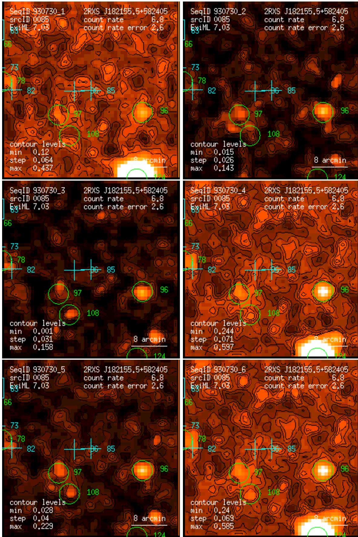
Figure 85: RASS 930730: detection 0085: band rate images, Gaussian filter: (1) PSPC channels 11 – 41, (2) 52 – 90, (3) 91 – 201, (4) 11 – 235, (5) 52 – 201, (6) 11 – 201. Broad band rates in counts/ks. Band rate contour levels in counts/ks/arcmin 2 .
