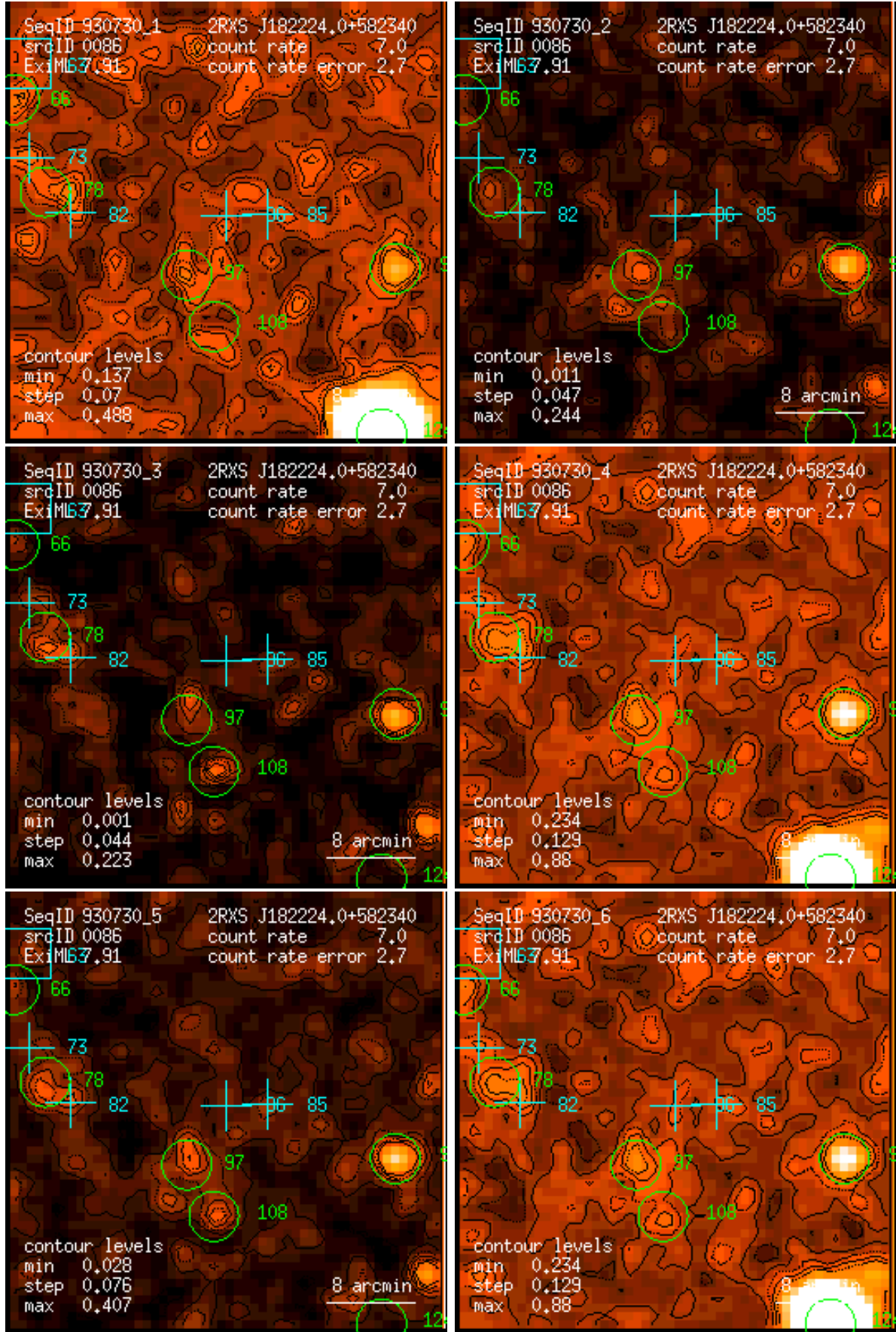
Figure 86: RASS 930730: detection 0086: band rate images, Gaussian filter: (1) PSPC channels 11 – 41, (2) 52 – 90, (3) 91 – 201, (4) 11 – 235, (5) 52 – 201, (6) 11 – 201. Broad band rates in counts/ks. Band rate contour levels in counts/ks/arcmin 2 .
