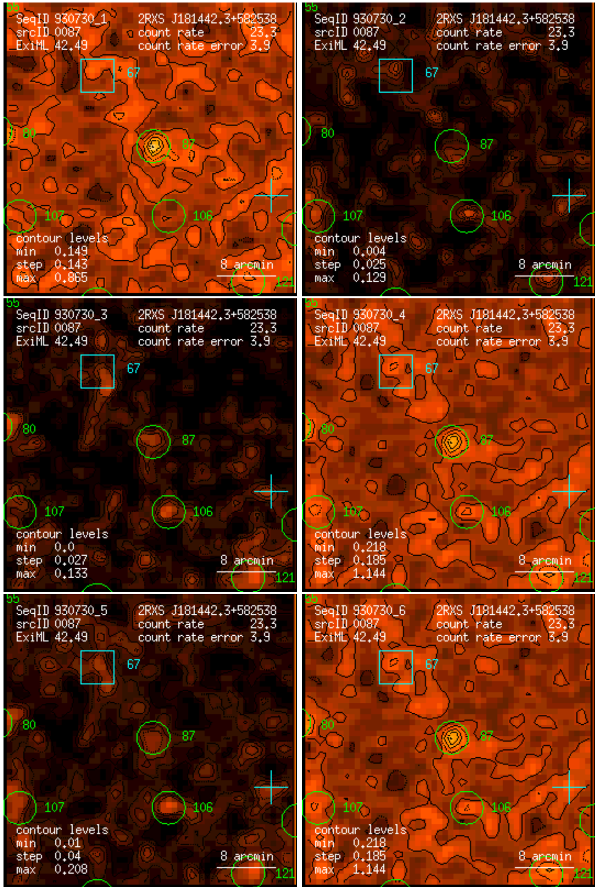
Figure 87: RASS 930730: detection 0087: band rate images, Gaussian filter: (1) PSPC channels 11 – 41, (2) 52 – 90, (3) 91 – 201, (4) 11 – 235, (5) 52 – 201, (6) 11 – 201. Broad band rates in counts/ks. Band rate contour levels in counts/ks/arcmin 2 .
