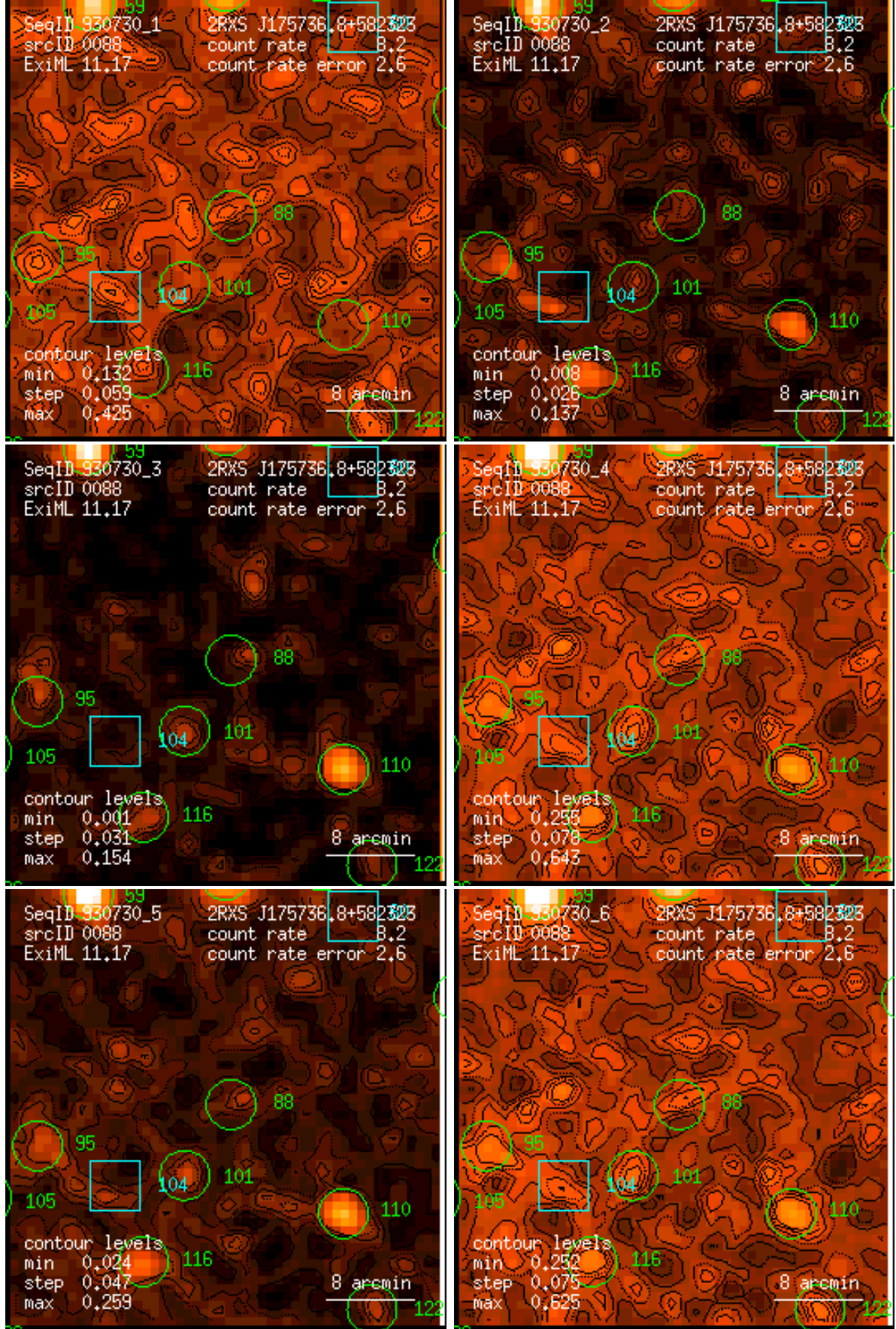
Figure 88: RASS 930730: detection 0088: band rate images, Gaussian filter: (1) PSPC channels 11 – 41, (2) 52 – 90, (3) 91 – 201, (4) 11 – 235, (5) 52 – 201, (6) 11 – 201. Broad band rates in counts/ks. Band rate contour levels in counts/ks/arcmin 2 .
