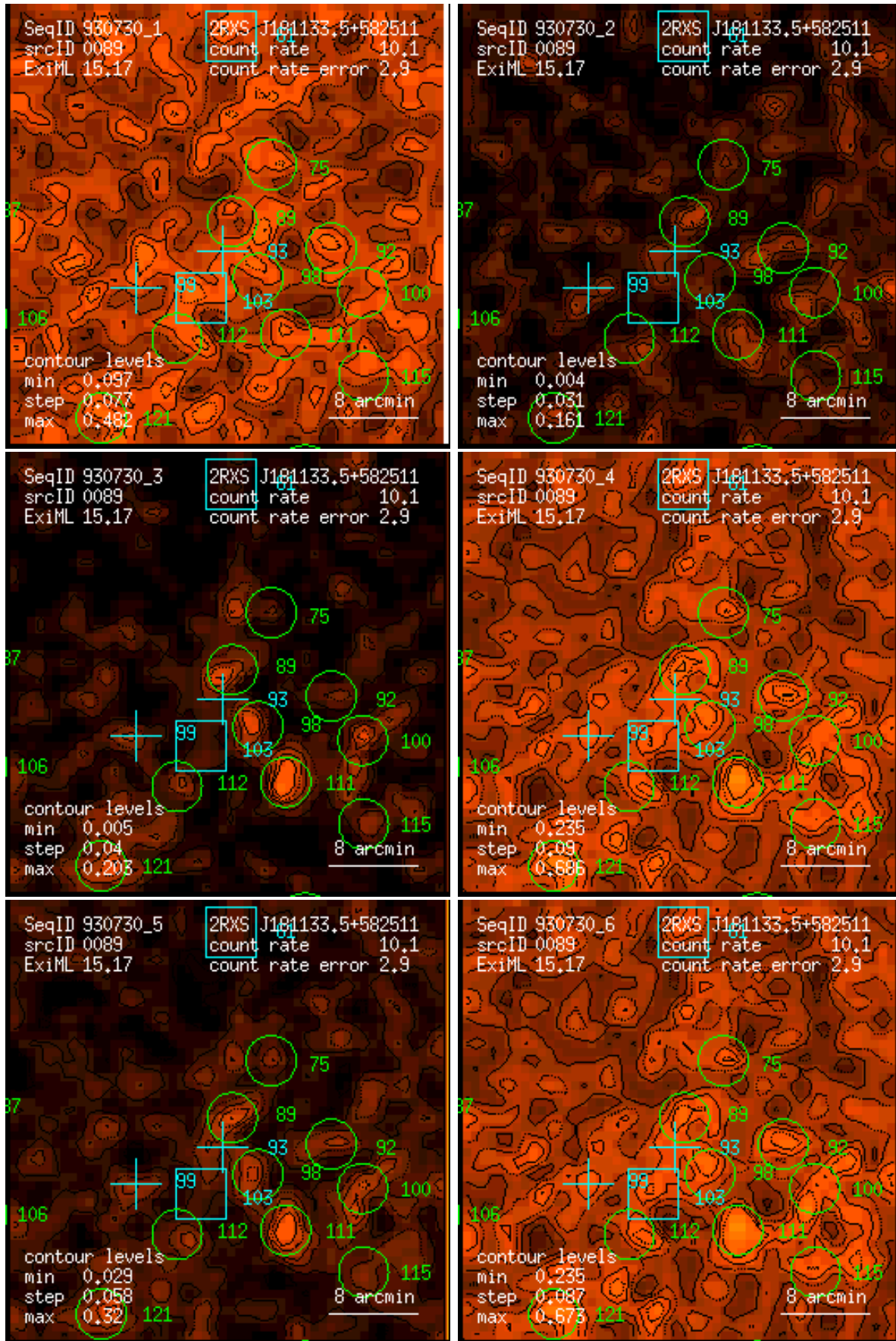
Figure 89: RASS 930730: detection 0089: band rate images, Gaussian filter: (1) PSPC channels 11 – 41, (2) 52 – 90, (3) 91 – 201, (4) 11 – 235, (5) 52 – 201, (6) 11 – 201. Broad band rates in counts/ks. Band rate contour levels in counts/ks/arcmin 2 .
