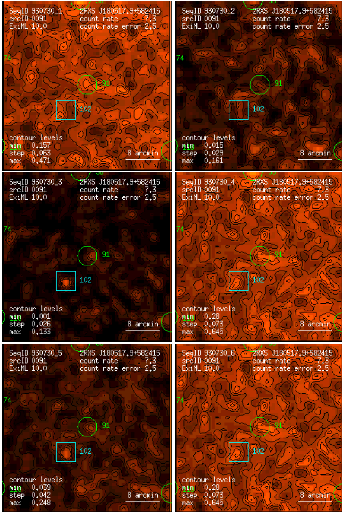
Figure 91: RASS 930730: detection 0091: band rate images, Gaussian filter: (1) PSPC channels 11 – 41, (2) 52 – 90, (3) 91 – 201, (4) 11 – 235, (5) 52 – 201, (6) 11 – 201. Broad band rates in counts/ks. Band rate contour levels in counts/ks/arcmin 2 .
