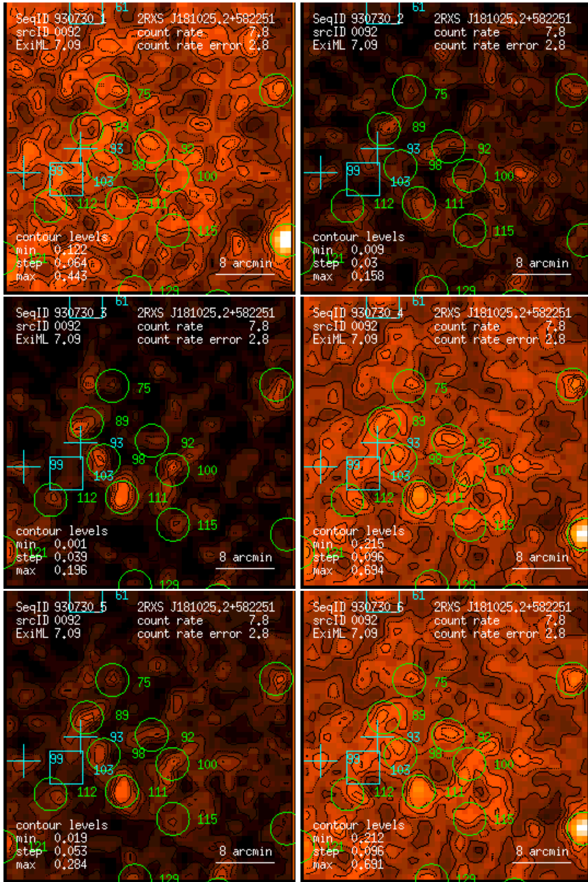
Figure 92: RASS 930730: detection 0092: band rate images, Gaussian filter: (1) PSPC channels 11 – 41, (2) 52 – 90, (3) 91 – 201, (4) 11 – 235, (5) 52 – 201, (6) 11 – 201. Broad band rates in counts/ks. Band rate contour levels in counts/ks/arcmin 2 .
