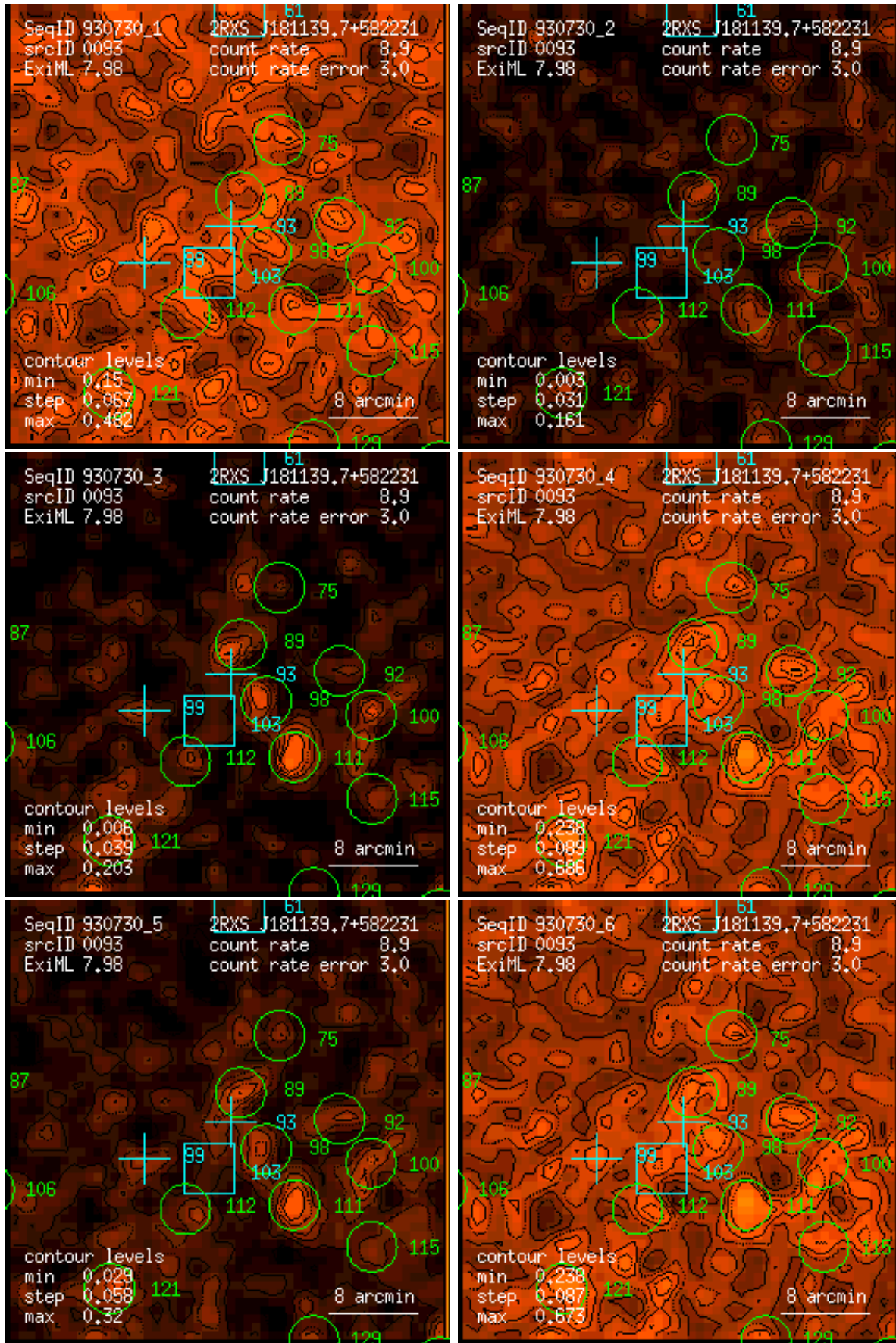
Figure 93: RASS 930730: detection 0093: band rate images, Gaussian filter: (1) PSPC channels 11 – 41, (2) 52 – 90, (3) 91 – 201, (4) 11 – 235, (5) 52 – 201, (6) 11 – 201. Broad band rates in counts/ks. Band rate contour levels in counts/ks/arcmin 2 .
