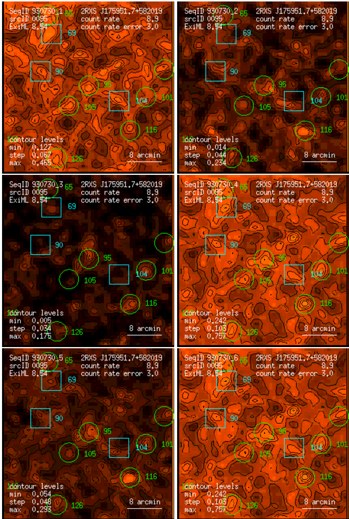
Figure 95: RASS 930730: detection 0095: band rate images, Gaussian filter: (1) PSPC channels 11 – 41, (2) 52 – 90, (3) 91 – 201, (4) 11 – 235, (5) 52 – 201, (6) 11 – 201. Broad band rates in counts/ks. Band rate contour levels in counts/ks/arcmin 2 .
