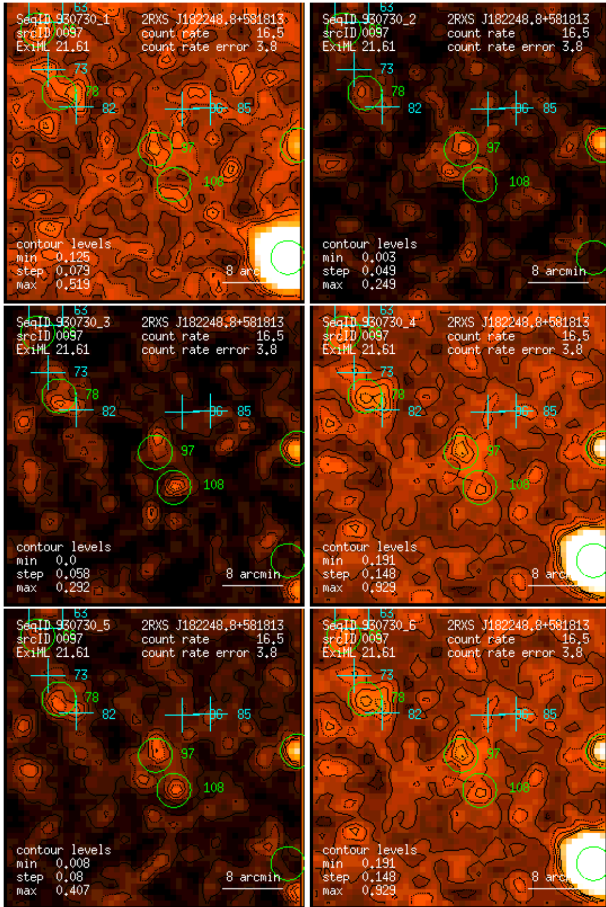
Figure 97: RASS 930730: detection 0097: band rate images, Gaussian filter: (1) PSPC channels 11 – 41, (2) 52 – 90, (3) 91 – 201, (4) 11 – 235, (5) 52 – 201, (6) 11 – 201. Broad band rates in counts/ks. Band rate contour levels in counts/ks/arcmin 2 .
