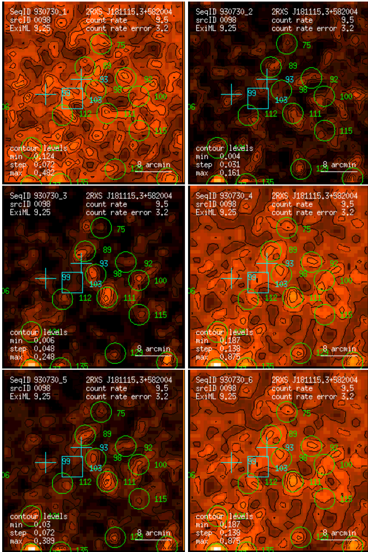
Figure 98: RASS 930730: detection 0098: band rate images, Gaussian filter: (1) PSPC channels 11 – 41, (2) 52 – 90, (3) 91 – 201, (4) 11 – 235, (5) 52 – 201, (6) 11 – 201. Broad band rates in counts/ks. Band rate contour levels in counts/ks/arcmin 2 .
